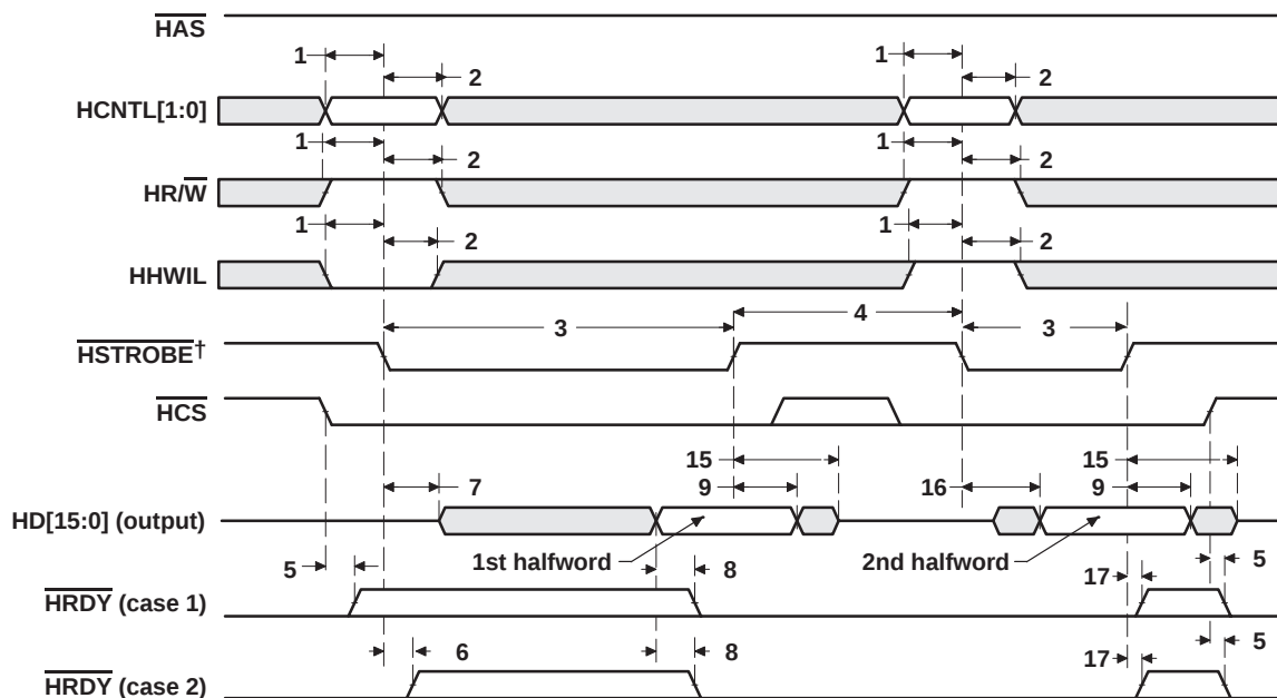
Figure 52. HPI Read Timing ( \overline{HAS} Not Used, Tied High)
