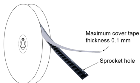
Figure 27. Tape and reel orientation
