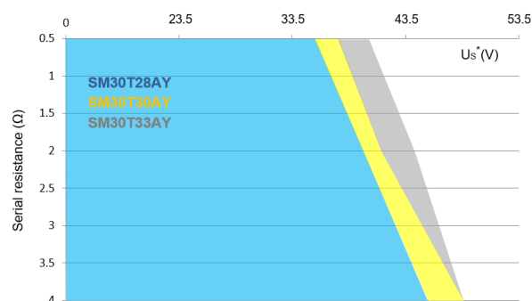
Figure 22. Load dump capability (typical values, U_s^* = f(R_i) test B, U_s = 87 V, t_p = 400 ms)
