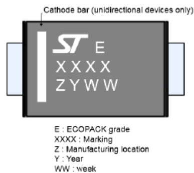
Figure 25. Marking layout
