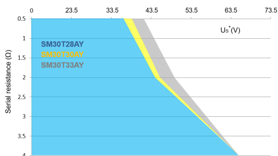
Figure 21. Load dump capability (typical values, U_s^* = f(R_i) test B, U_s = 87 V, t_p = 150 ms)
