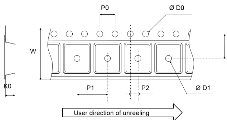
Figure 30. Tape outline
