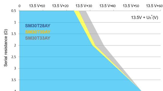
Figure 18. Load dump capability (typical values, U_s^* = f(R_i) pulse 5b, U_s = 87 V, t_p = 150 ms)
