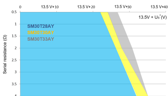
Figure 19. Load dump capability (typical values, U_s^* = f(R_i) pulse 5b, U_s = 87 V, t_p = 400 ms)
