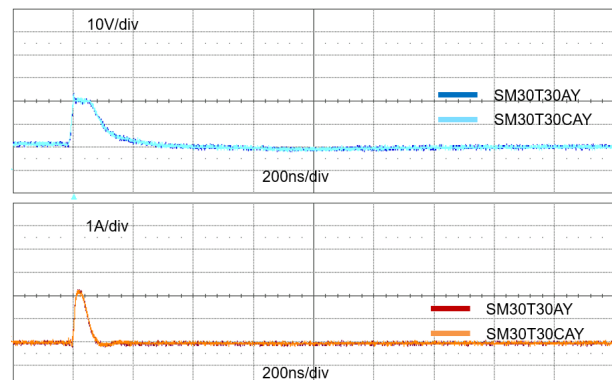
Figure 16. ISO7637-2 pulse 3b response ( V_S = 150\text{ V} ) with 12 V battery
