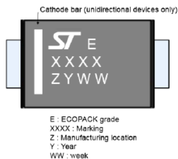
Figure 15. Marking layout
