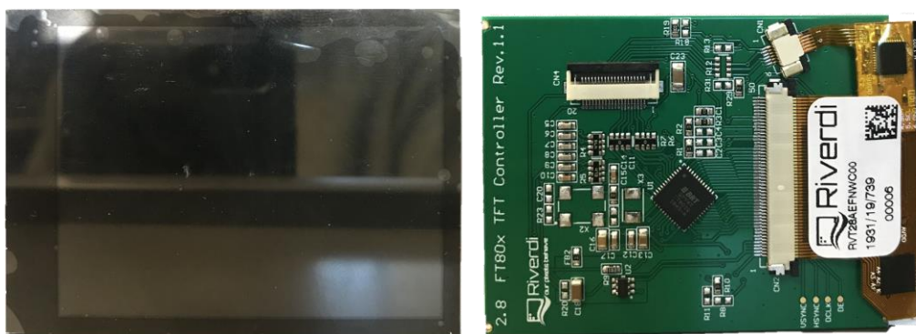
Figure 52: Riverdi Display
