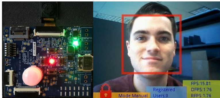
Figure 7: Face Detected
