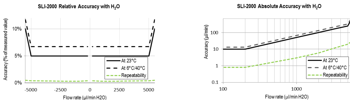
Figure 1 (cont.): Flow meter accuracy and repeatability across the flow range. Relative error in % of measured value (left column) and absolute error in μl/min (right column) for H 2 O
