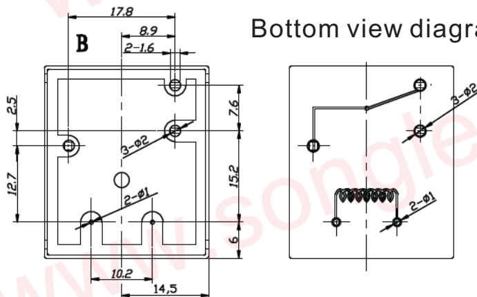
Bottom view diagram B Tolerance: \pm 0.1\text{mm}
