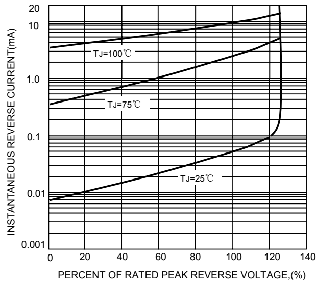
FIG.2-TYPICAL REVER CHARACTERISTICS
