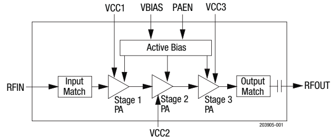
Figure 1. SKY66293-21 Block Diagram
