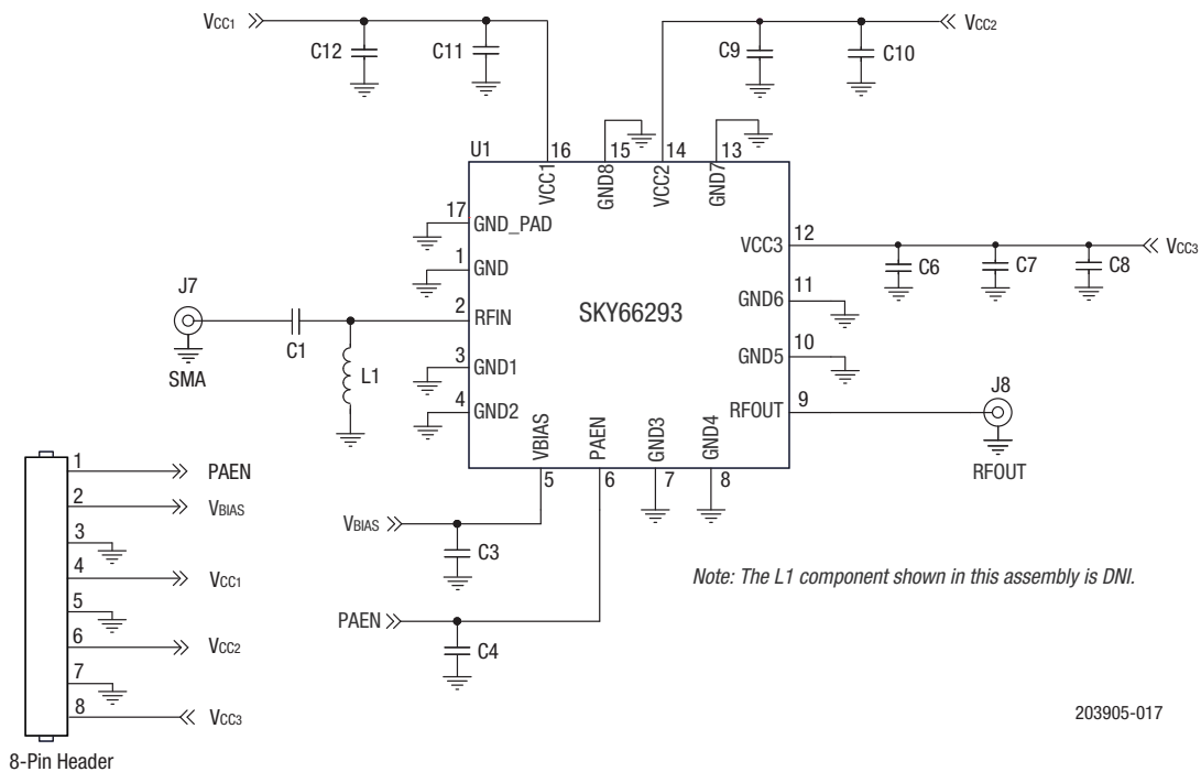
Figure 17. SKY66293-21 Evaluation Board Schematic
