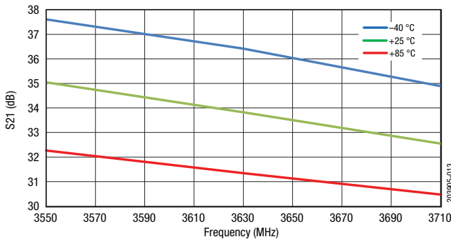
Figure 13. Small Signal Gain vs Frequency Across Temperature (PIN = -20 dBm)
