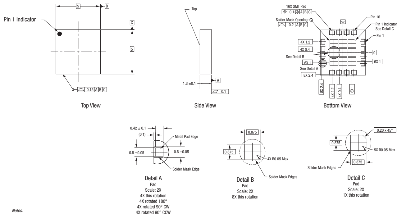
Figure 23. SKY66293-21 Package Dimensions
