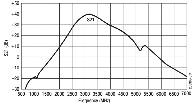
Figure 14. Wide Band Small Signal Gain vs Frequency
