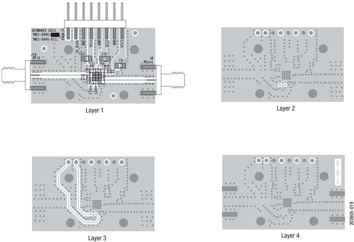
Figure 19. Board Layer Detail
