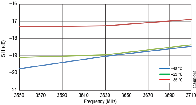
Figure 15. Input Return Loss vs Frequency Across Temperature (Small Signal, PIN = -20 dBm)
