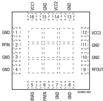
Figure 2. SKY66293-21 Pinout (Top View)
