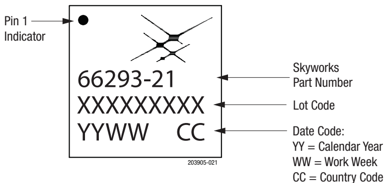
Figure 21. Typical Part Marking for the SKY66293-21
