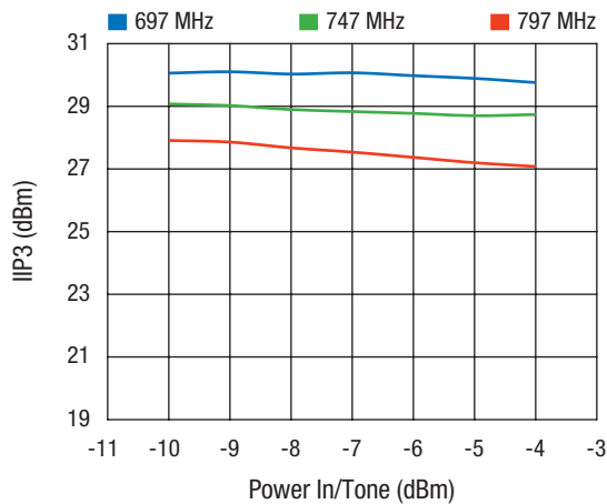
IIP3 vs. Power In/Tone Across Frequency
