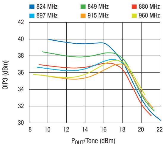
OIP3 vs. P_{OUT}/\text{Tone} Across Frequency
