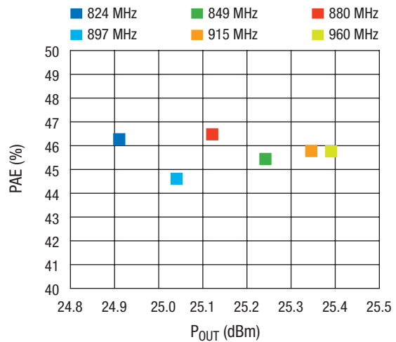
PAE @ P_1\text{ dB} vs. P_{OUT} Across Frequency
