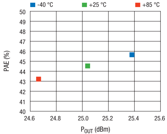
PAE @ P_1\text{ dB} vs. P_{OUT} Across Temperature
