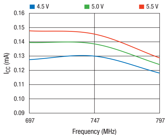
I_{CC} @ P_1\text{ dB} vs. Frequency Across V_{CC}
