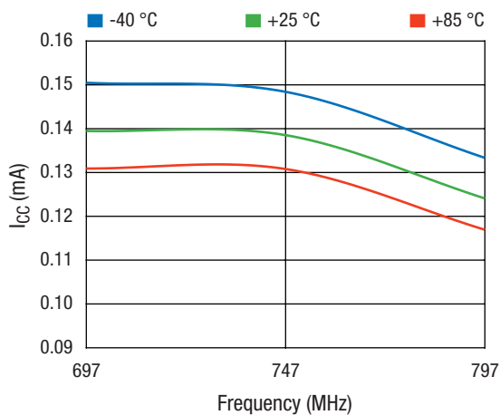
I_{CC} @ P_1\text{ dB} vs. Frequency Across Temperature
