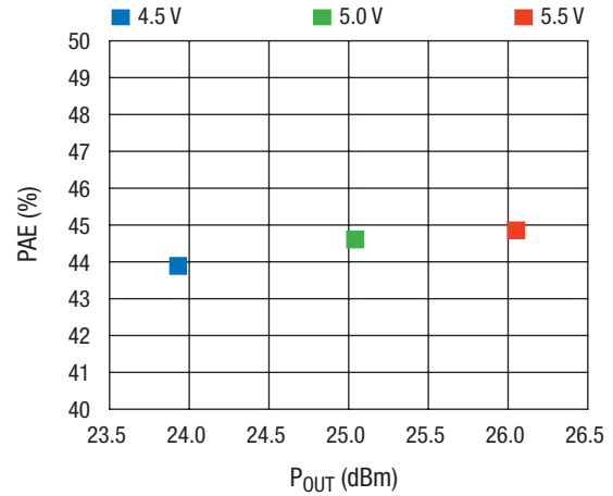
PAE @ P_1\text{ dB} vs. P_{OUT} Across V_{CC}
