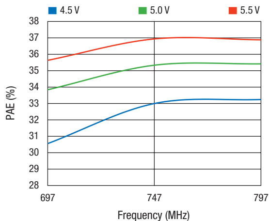
PAE @ P_1\text{ dB} vs. Frequency Across V_{CC}
