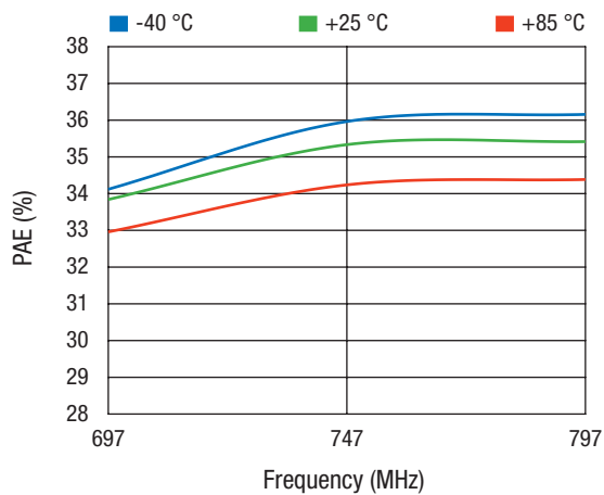
PAE @ P_1\text{ dB} vs. Frequency Across Temperature
