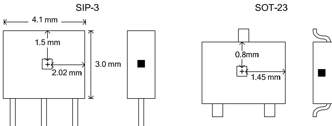
Fig. 1 SENSOR LOCATIONS
