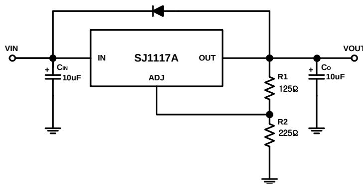
Fig.2 Adjustable Voltage Regulator
