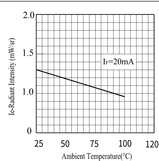
Relative Intensity vs Ambient Temperature(°C)
