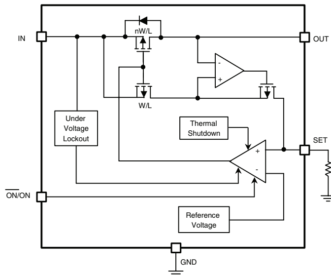
Figure 1. SiP4612A/B Block Diagram
