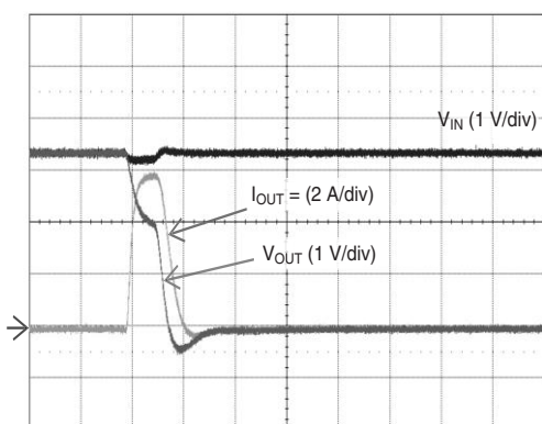
Short Circuit through 0.3 \Omega , V_{in} = 3.3 V
