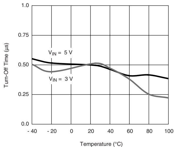
Turn-Off vs. Temperature R_L = 10\ \Omega , C_L = 0.47\ \mu\text{F}
