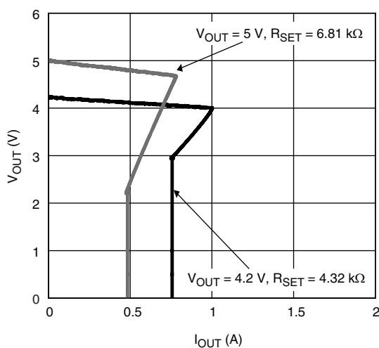
Output Current vs. V_{\text{OUT}}
