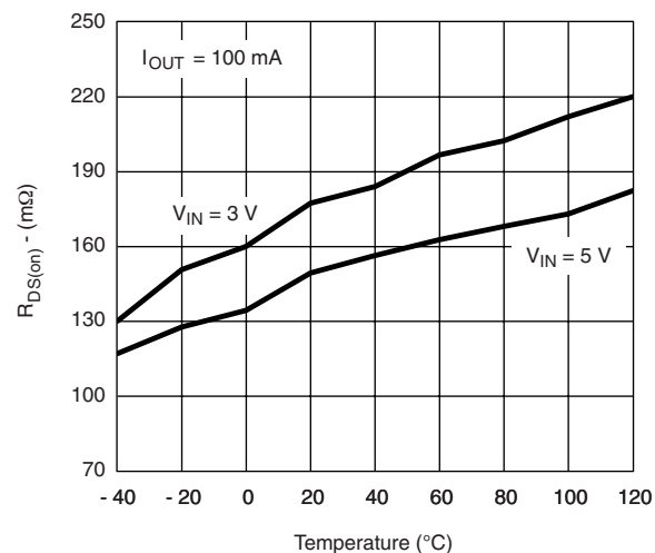
R_{\text{DS(on)}} vs. Temperature
