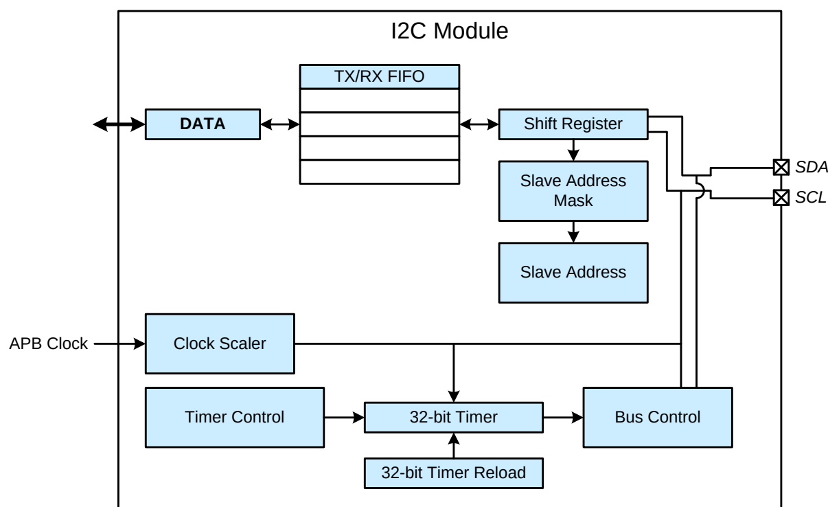
Figure 25.1. I2C Block Diagram
