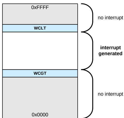
Figure 34.10. Example Window Comparator Limits for Inside Range (WCGT < WCLT)
