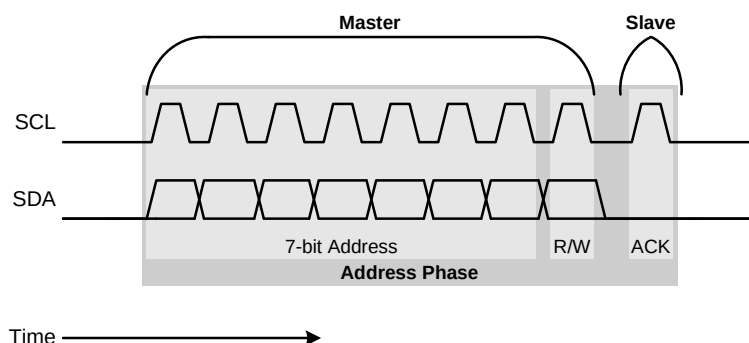
Figure 25.4. I2C 7-bit Address Phase
