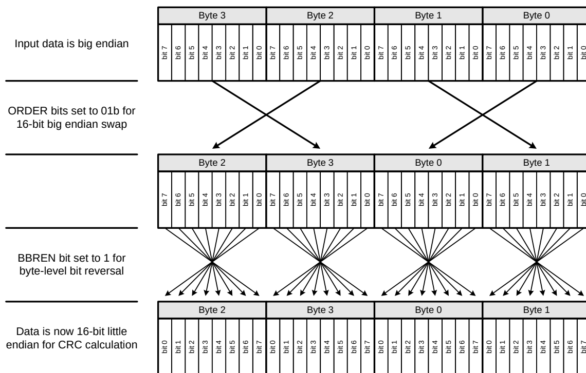
Figure 20.5. Data Ordering Example—Big Endian to 16-bit Little Endian
