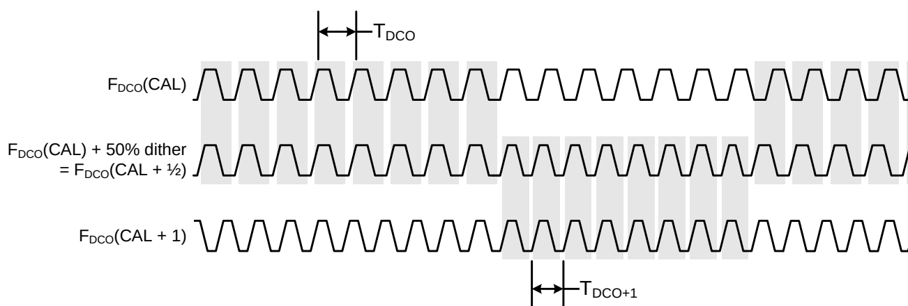
Figure 31.6. Dithering Timing Example
