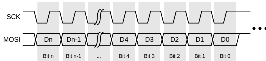
Figure 35.3. SPI Clock Polarity and Phase Combinations (DDIRSEL = 0, Master Mode)
