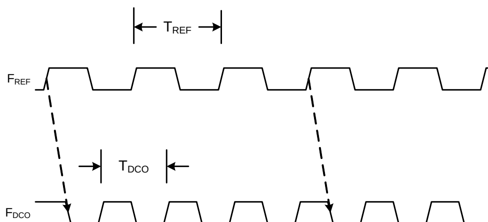
Figure 31.3. Frequency-Lock Mode
