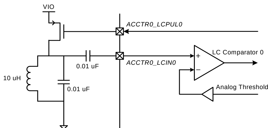
Figure 14.9. LC Resonant Example Schematic
