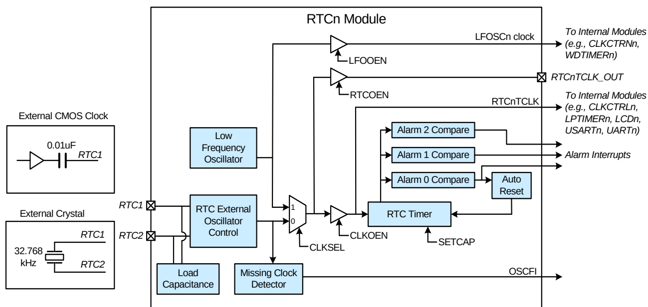
Figure 33.1. RTC Block Diagram
