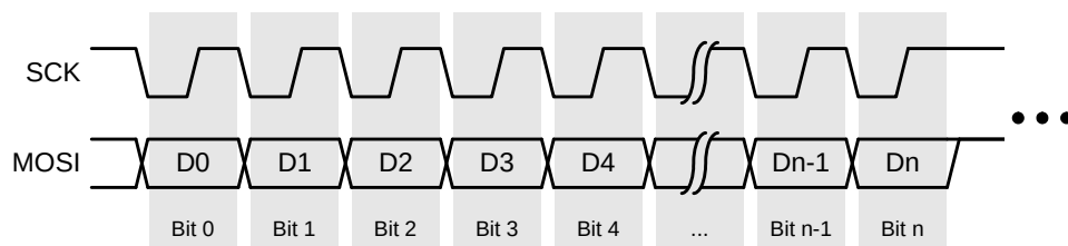
Figure 35.4. SPI Clock Polarity and Phase Combinations (DDIRSEL = 1, Master Mode)
