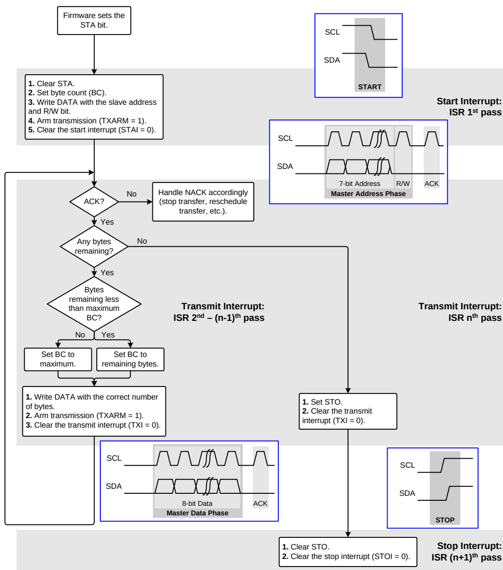
Figure 25.8. Master Write Flow Diagram (7-bit Address)
