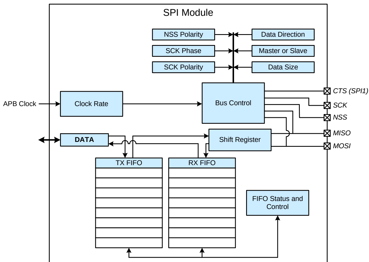
Figure 35.1. SPI Block Diagram
