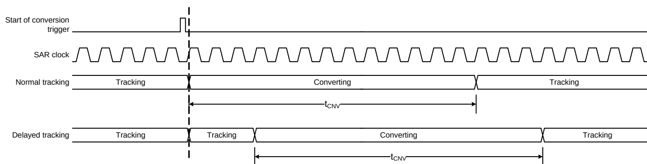
Figure 34.3. Non-Burst Tracking and Conversion Timing
