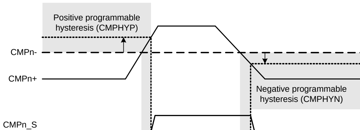
Figure 16.7. Comparator Hysteresis
