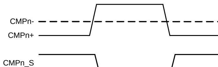
Figure 16.6. Output Configurations
