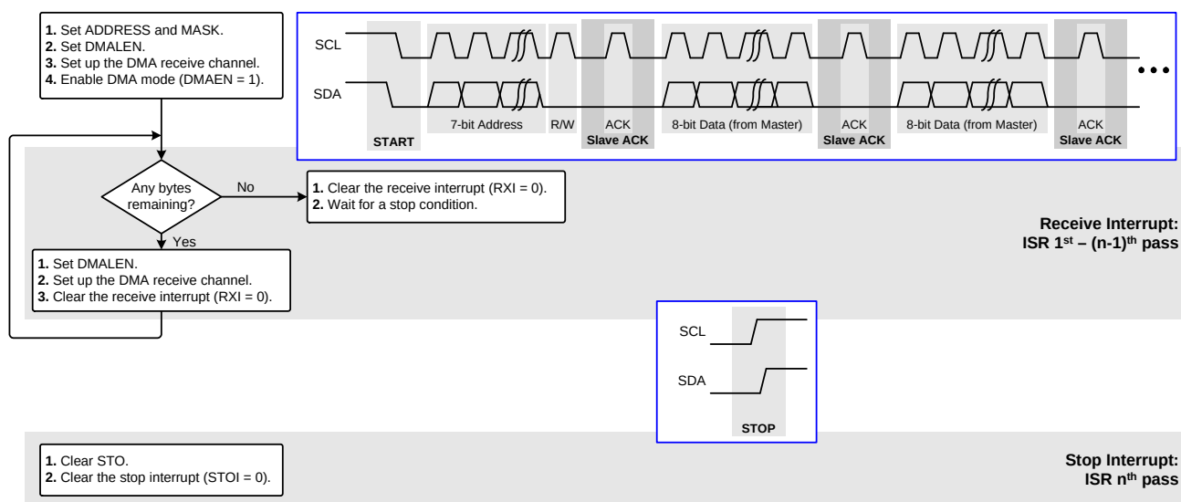
Figure 25.19. Slave Write with DMA and Automatic Hardware Flow Diagram (7-bit Address)
