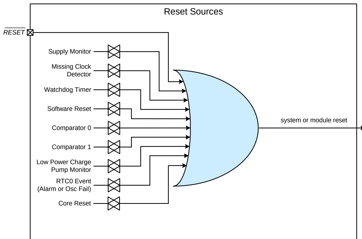
Figure 7.1. Reset Sources Block Diagram
