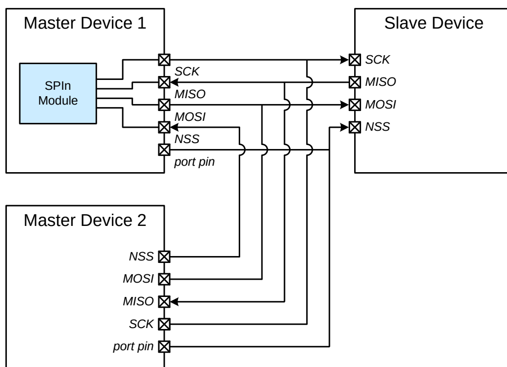
Figure 35.8. 4-Wire Multiple Master Mode Connection Diagram
