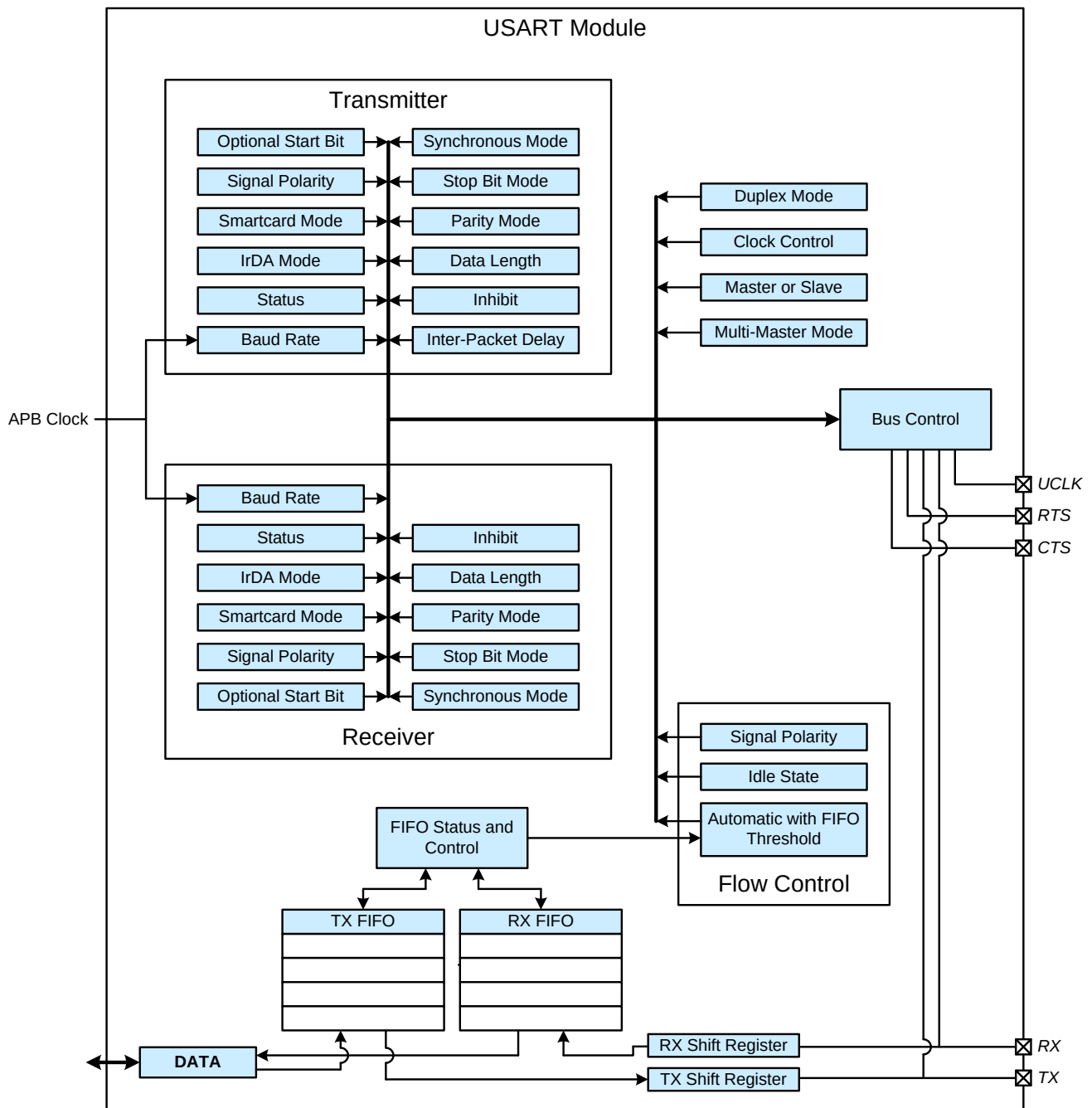
Figure 37.1. USART Block Diagram
