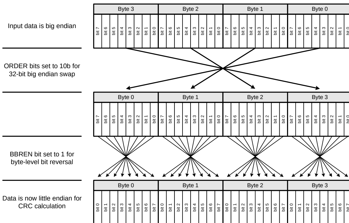
Figure 20.4. Data Ordering Example—Big Endian to Little Endian
