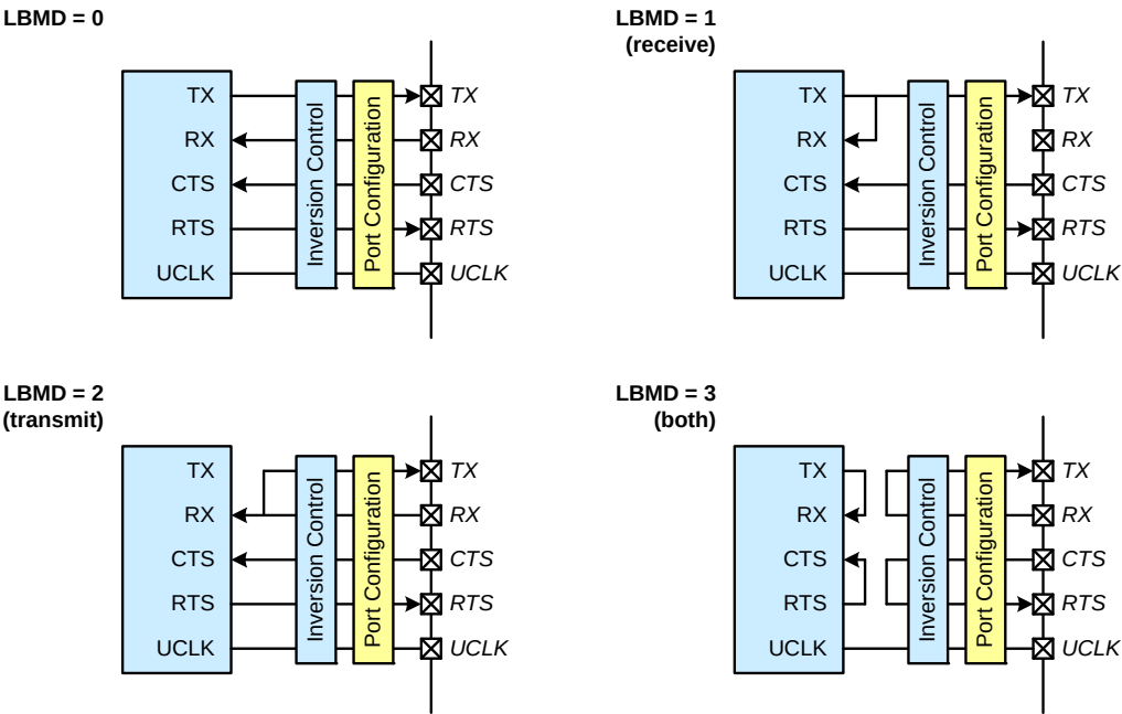
Figure 37.9. Internal Loop Back Connections
