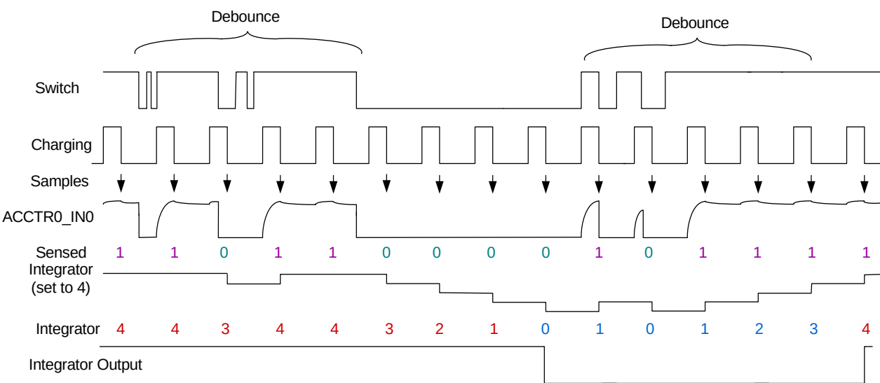
Figure 14.8. Debounce Timing
