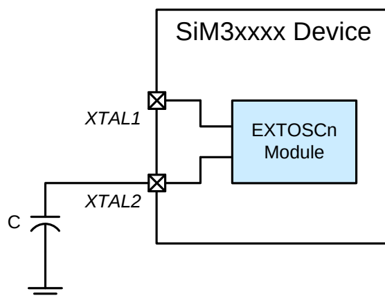
Figure 23.4. External C Oscillator Configuration
