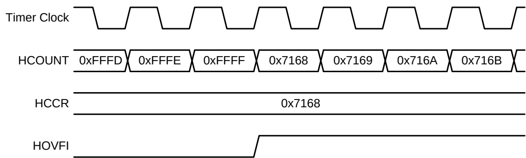
Figure 36.8. 16-bit Auto-Reload Mode Timing Diagram
