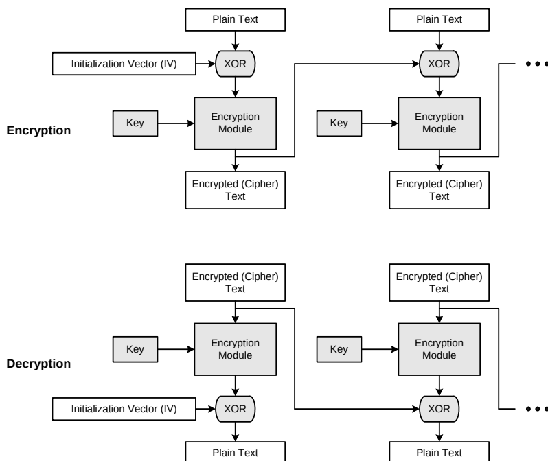
Figure 15.5. Cipher Block Chaining (CBC) Algorithm Diagram
