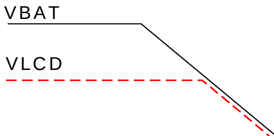
Figure 27.6. Contrast Control Mode 4
