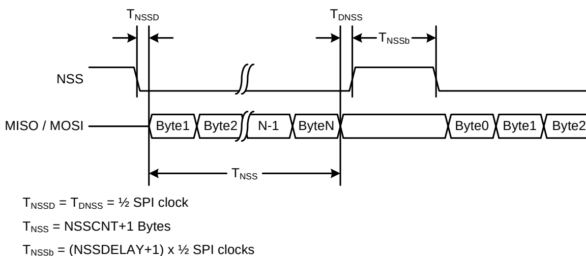
Figure 35.7. NSS Timing with AUTONSS = 1
