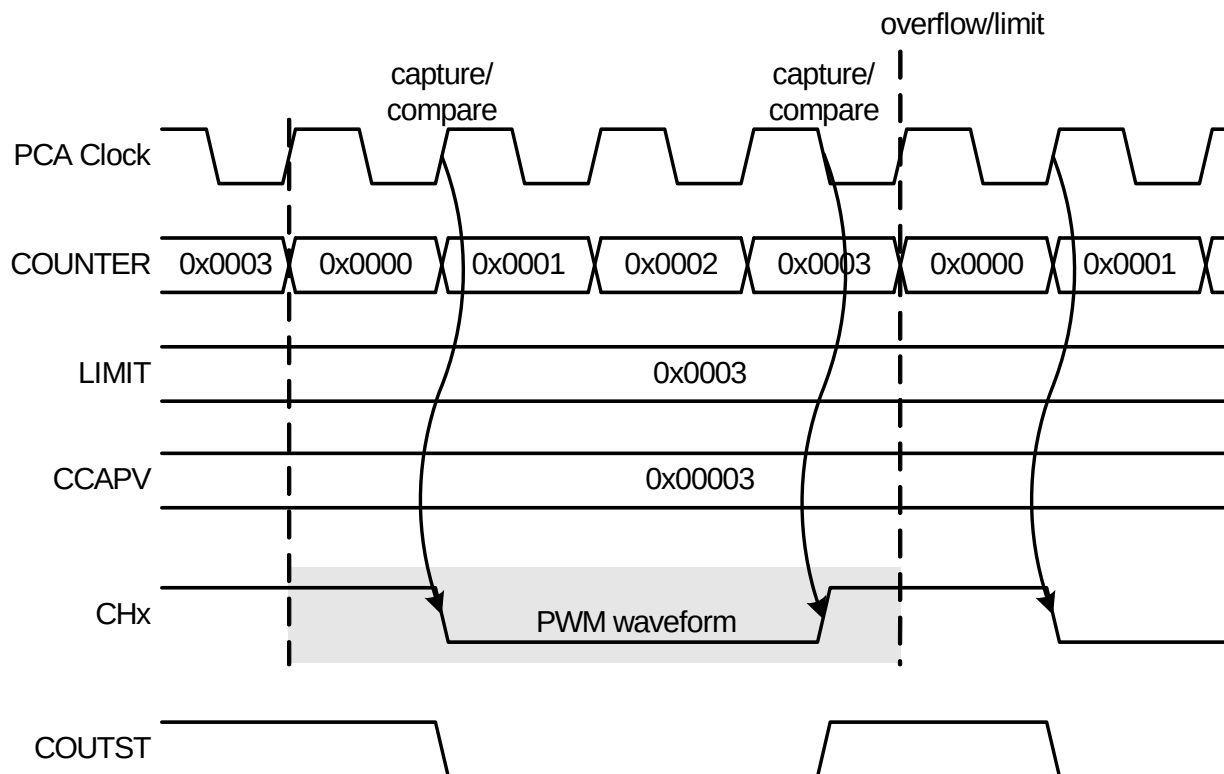
Figure 22.8. Example Center-Aligned PWM Timing Diagram
