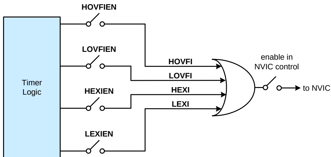
Figure 36.4. Timer Interrupt Configuration
