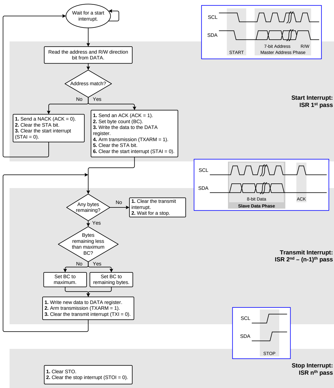
Figure 25.15. Slave Read Flow Diagram (7-bit Address)
