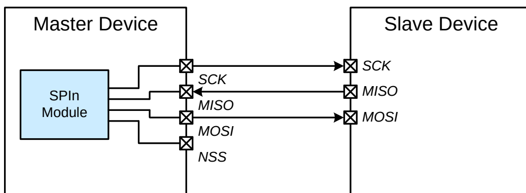
Figure 35.5. 3-Wire Single Master Mode Connection Diagram
