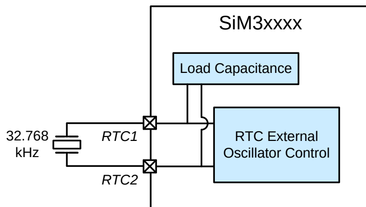
Figure 33.2. Crystal Mode Hardware Configuration
