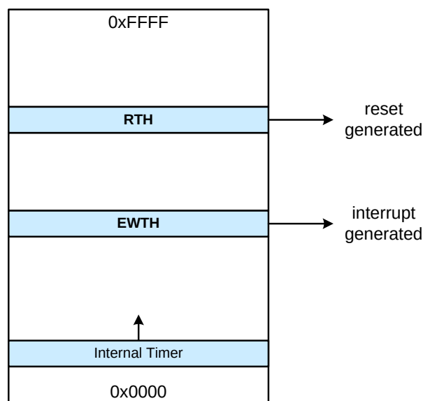
Figure 41.2. Early Warning and Reset Thresholds
