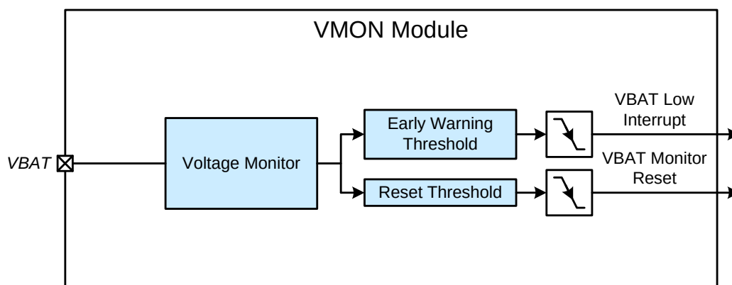
Figure 39.1. Voltage Supply Monitor Block Diagram
