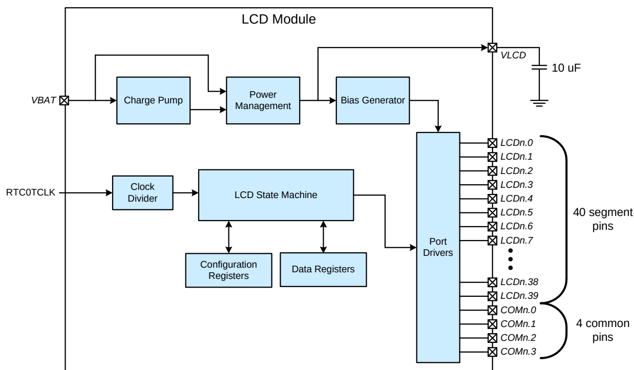
Figure 27.1. LCD0 Block Diagram
