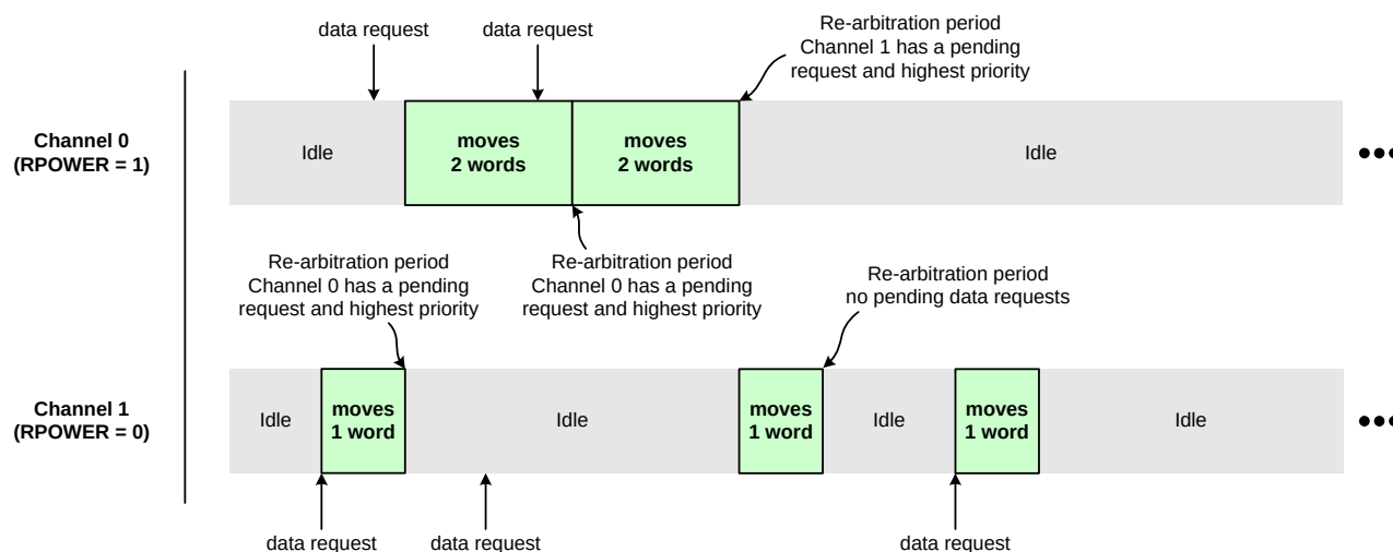
Figure 17.7. DMA Arbitration Example
