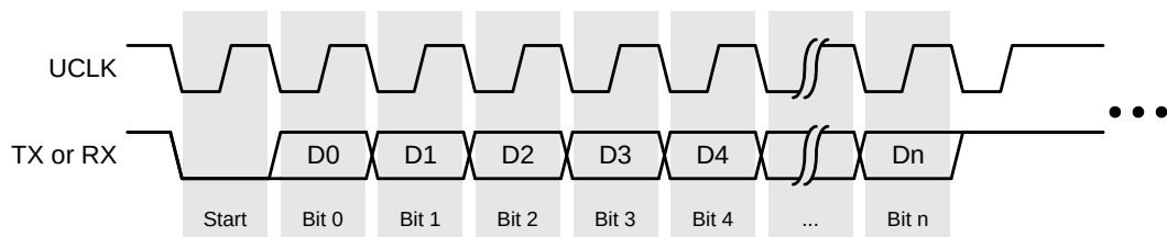
Figure 37.5. Clock Configurations
