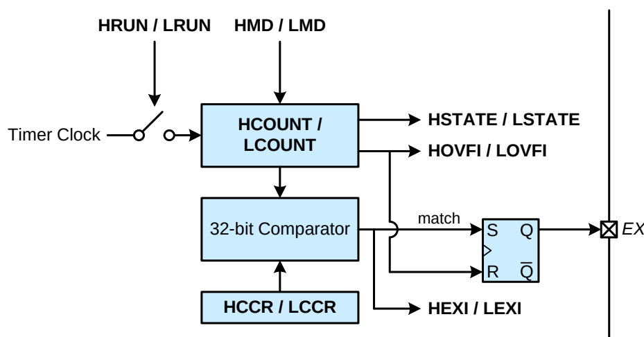
Figure 36.21. PWM Mode Block Diagram
