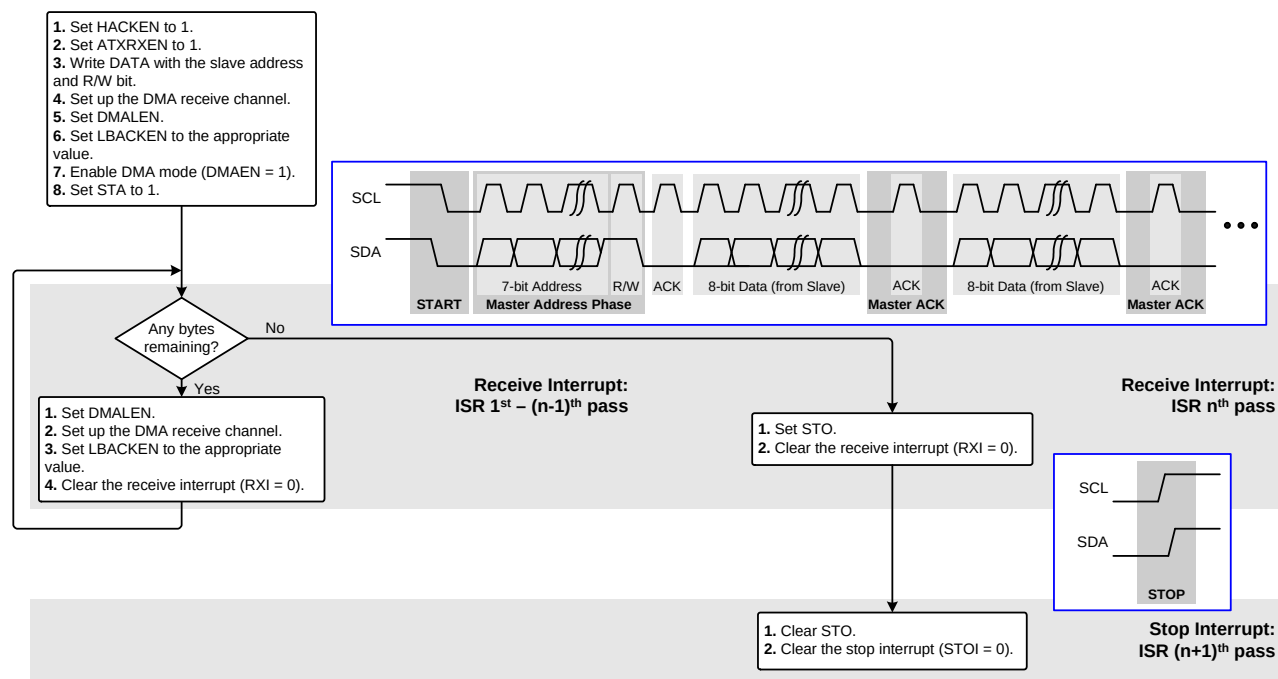
Figure 25.18. Master Read with DMA and Automatic Hardware Flow Diagram (7-bit Address)
