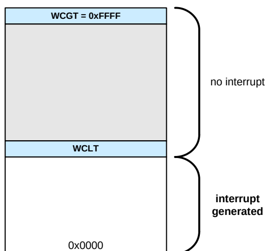
Figure 34.13. Example Window Comparator Limits for Below Value (WCLT = Value, WCGT = Full Scale)
