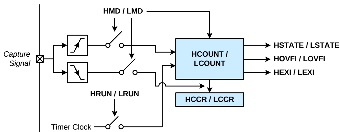
Figure 36.15. Duty Cycle Capture Mode Block Diagram
