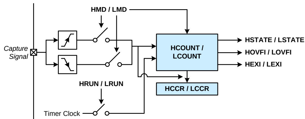
Figure 36.13. Pulse Capture Mode Block Diagram
