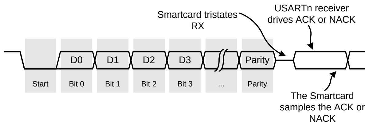
Figure 37.8. Smartcard Receive Signalling
