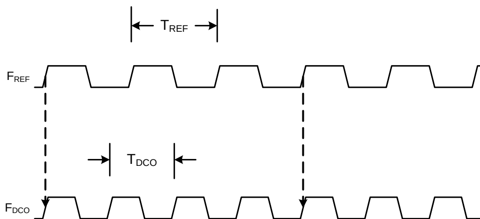
Figure 31.4. Phase-Lock Mode
