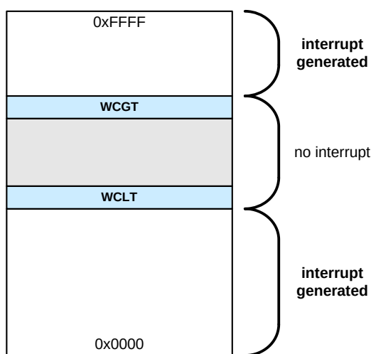
Figure 34.11. Example Window Comparator Limits for Outside Range (WCGT > WCLT)
