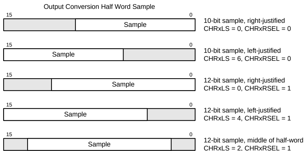
Figure 34.8. Sample Formatting
