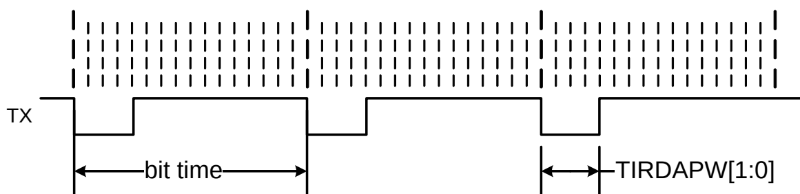
Figure 37.6. Transmit IrDA Pulse Width Timing
