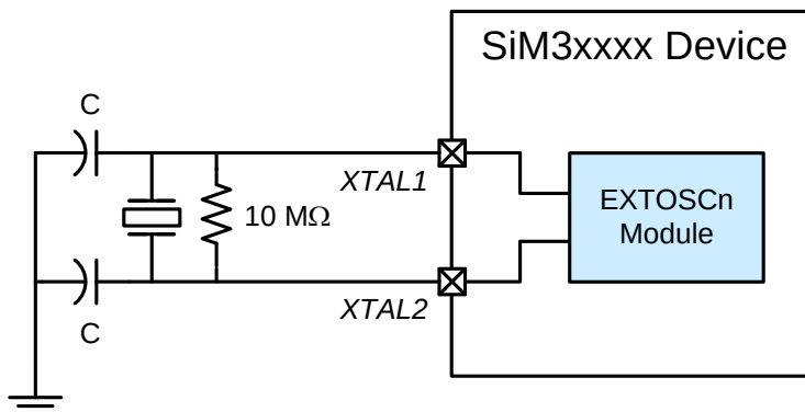
Figure 23.2. External Crystal Oscillator Configuration
