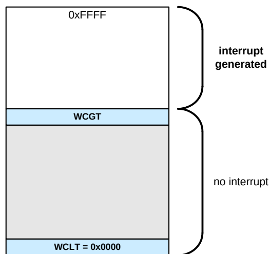
Figure 34.12. Example Window Comparator Limits for Above Value (WCGT = Value, WCLT = 0)
