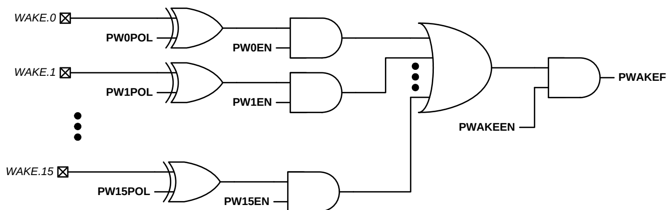
Figure 10.2. Pin Wake Logic
