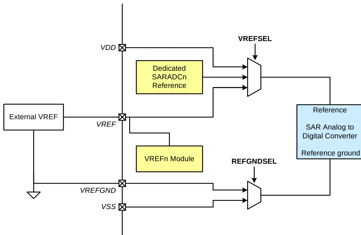
Figure 34.7. Voltage Reference Options
