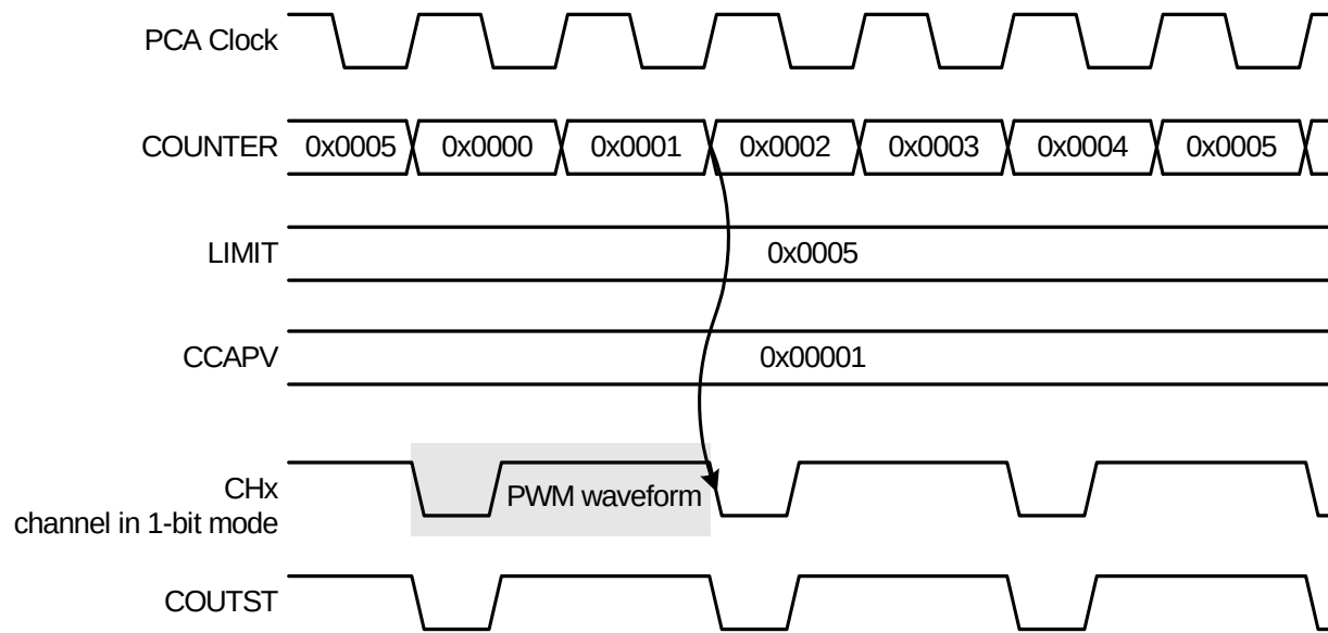
Figure 22.13. Example N-bit Edge-Aligned PWM Timing Diagram
