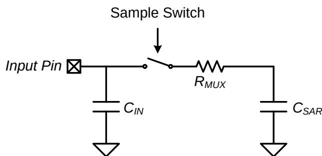
Figure 34.2. SARADC Input Model
