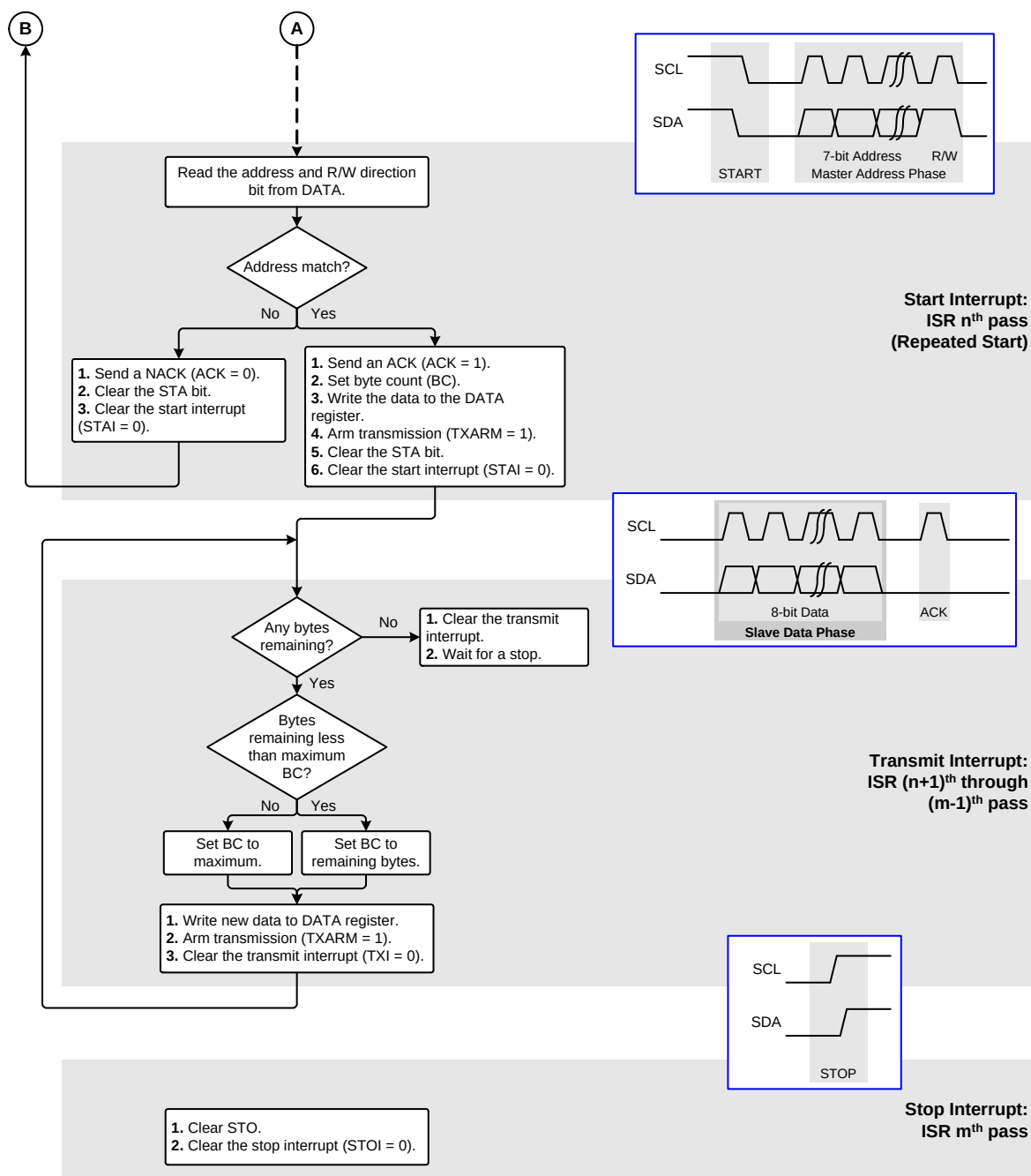
Figure 25.13. Slave Repeated Start (Write/Read) Flow Diagram (7-bit Address) (Page 2/2)
