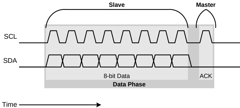
Figure 25.6. Single Byte I2C Read Data Phase
