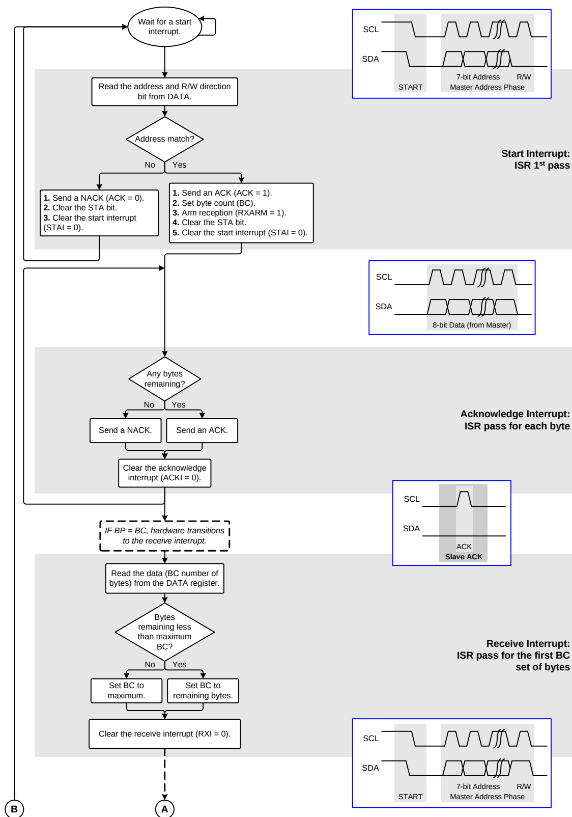
Figure 25.12. Slave Repeated Start (Write/Read) Flow Diagram (7-bit Address) (Page 1/2)
