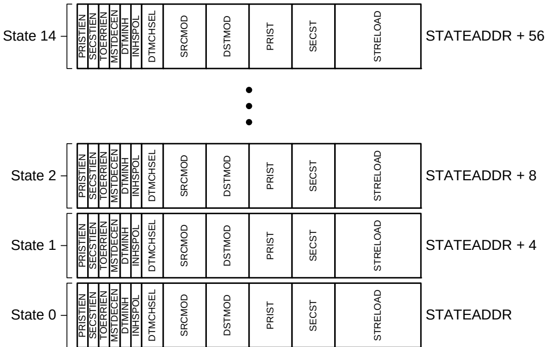
Figure 19.3. State Memory Map
