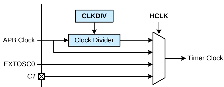
Figure 36.2. Clock Source Selection (SPLITEN = 0)
