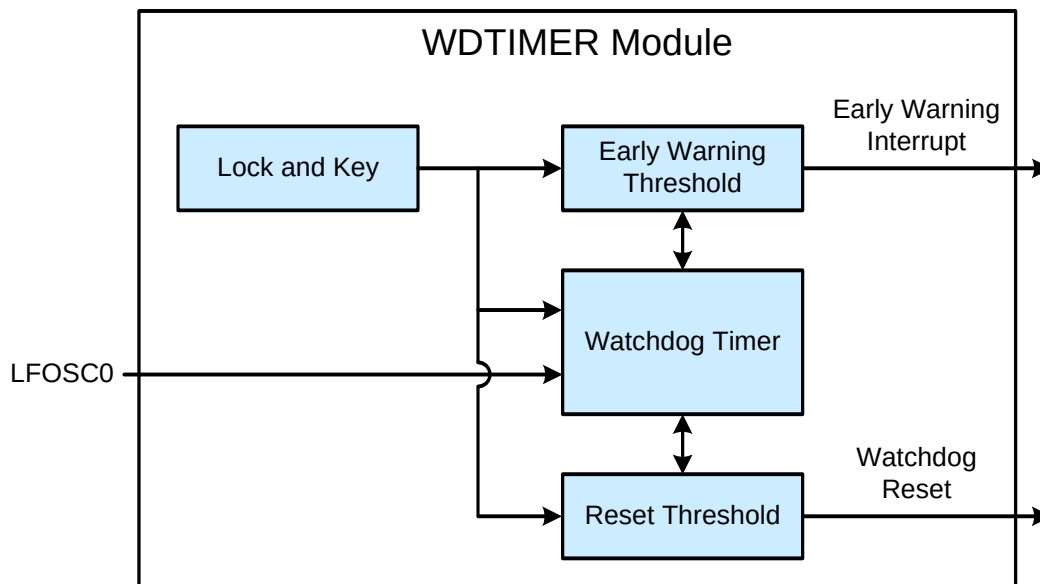
Figure 41.1. Watchdog Timer Block Diagram
