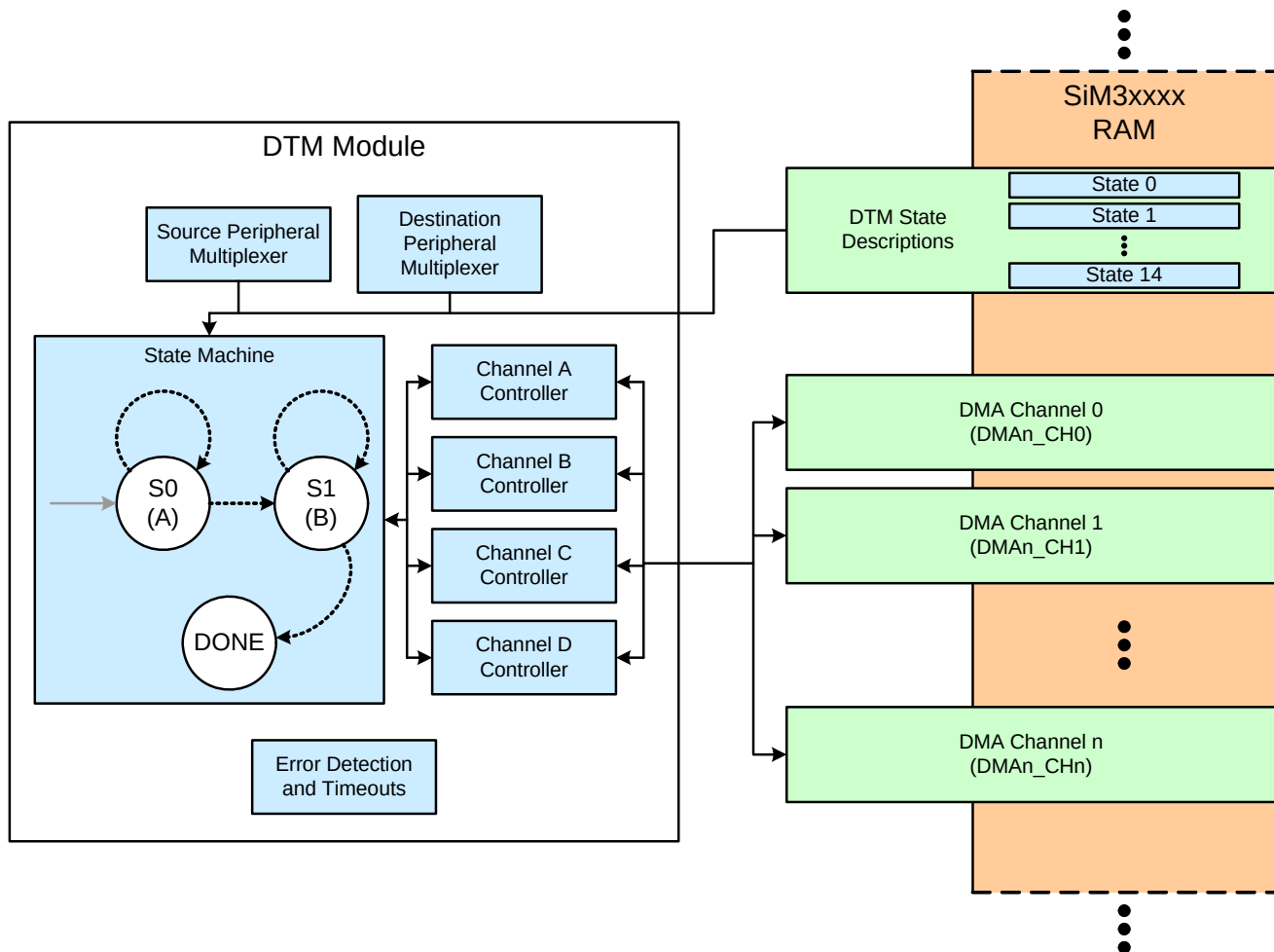
Figure 19.1. DTM Block Diagram
