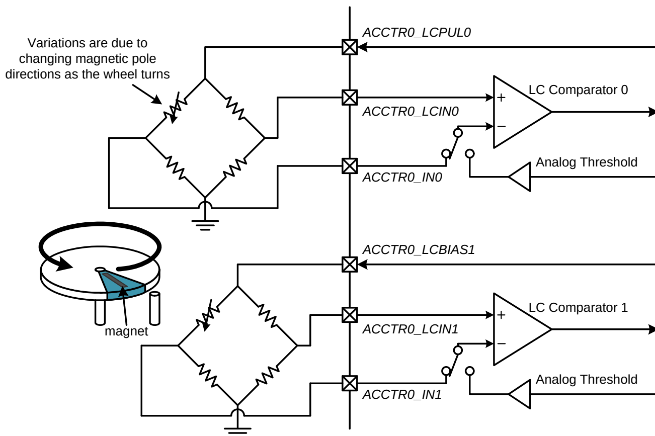
Figure 14.4. Wheatstone Bridge Configuration
