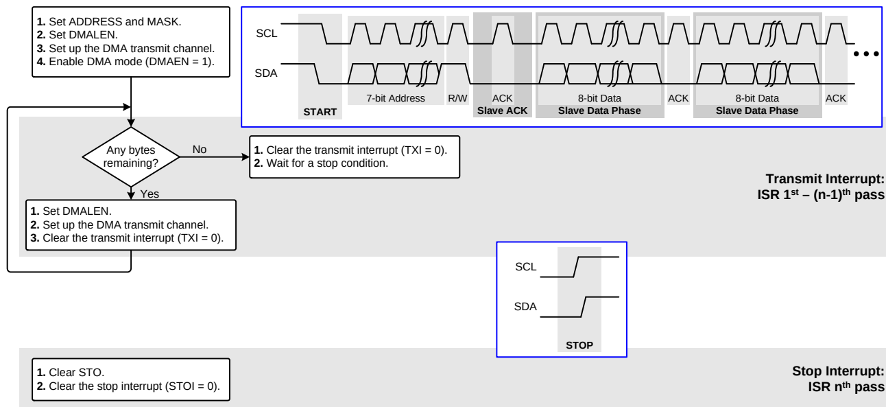
Figure 25.20. Slave Read with DMA and Automatic Hardware Flow Diagram (7-bit Address)
