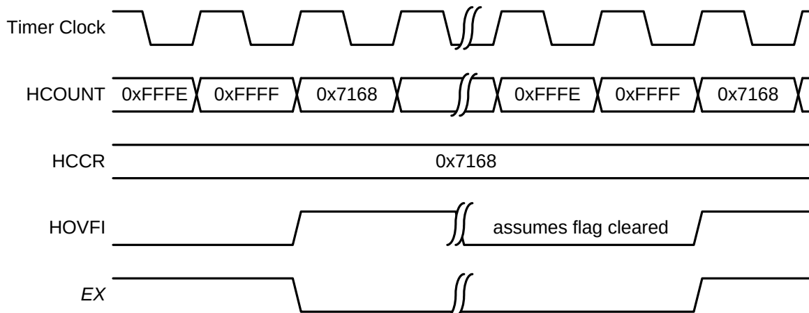
Figure 36.20. Square Wave Output Mode Timing Diagram
