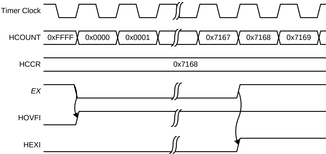
Figure 36.22. PWM Mode Timing Diagram
