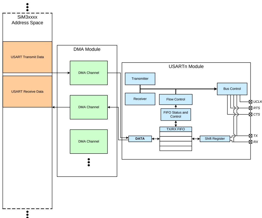
Figure 37.10. DMA Configuration
