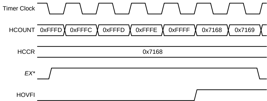
Figure 36.10. 16-bit Up/Down Mode Timing Diagram
