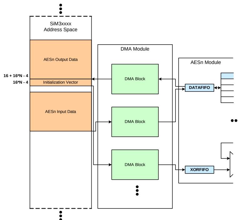
Figure 15.10. DMA XOR Channel Cipher Block Chaining Memory Setup
