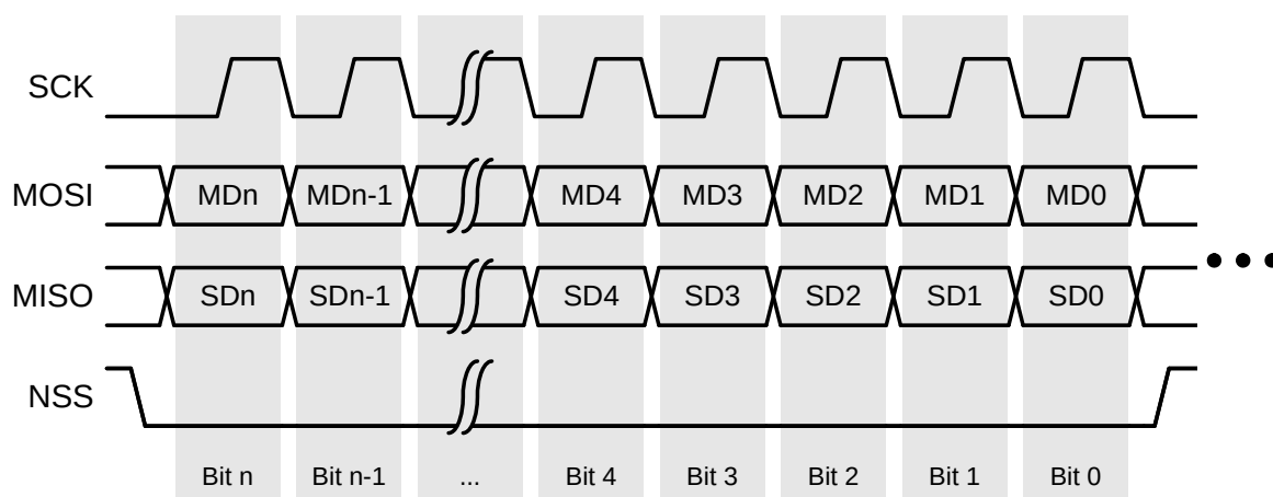
Figure 35.2. 4-Wire SPI Transfer
