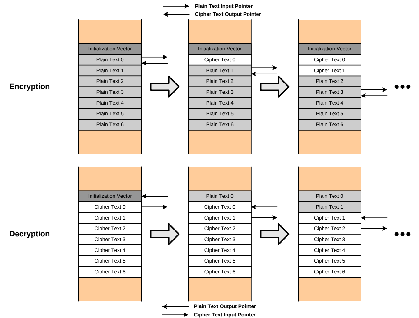
Figure 15.13. Memory Map of Hardware CBC Algorithm Performed In Place
