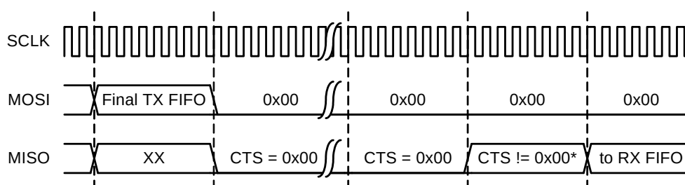
Figure 35.11. CTS Data Polling
