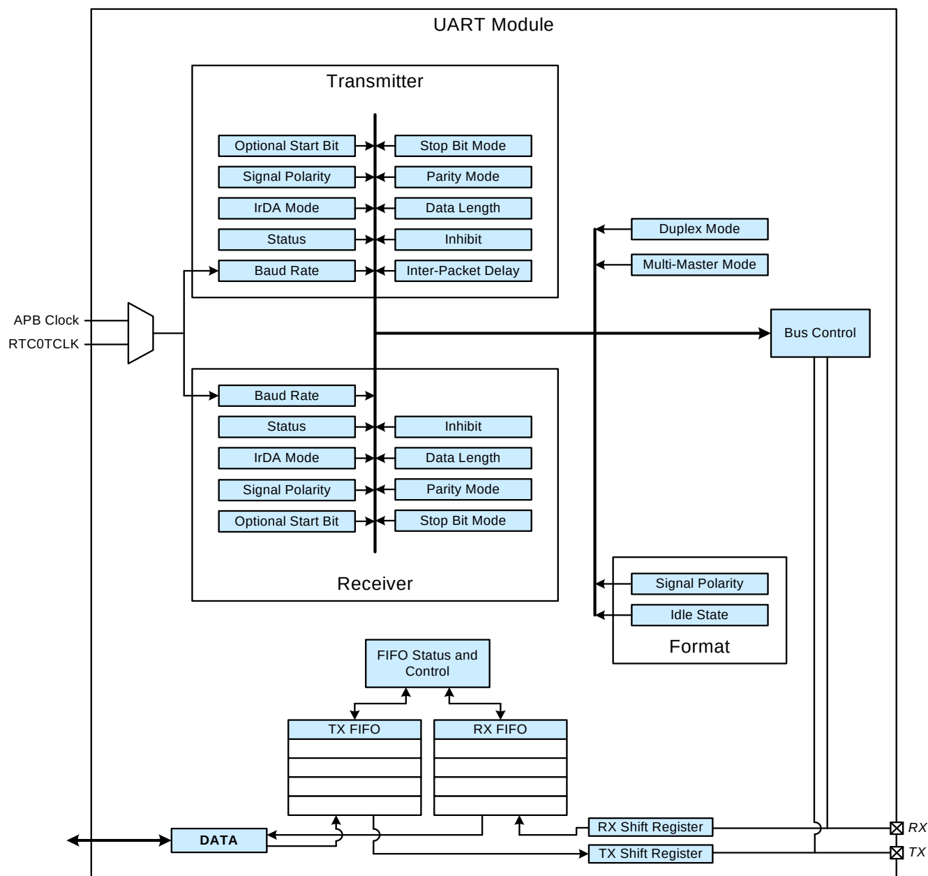
Figure 38.1. UART Block Diagram
