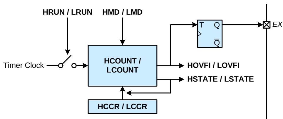
Figure 36.19. Square Wave Output Mode Block Diagram
