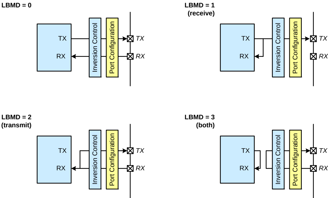
Figure 38.5. Internal Loop Back Connections
