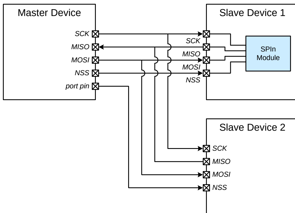
Figure 35.10. 4-Wire Slave Mode Connection Diagram
