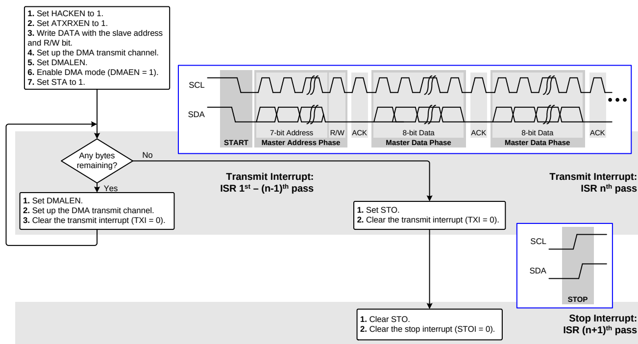
Figure 25.17. Master Write with DMA and Automatic Hardware Flow Diagram (7-bit Address)
