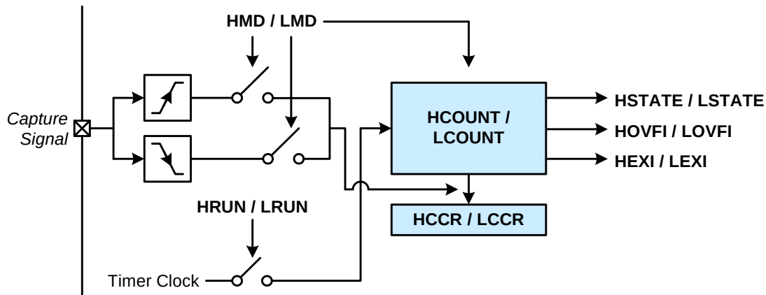
Figure 36.11. Edge Capture Mode Block Diagram
