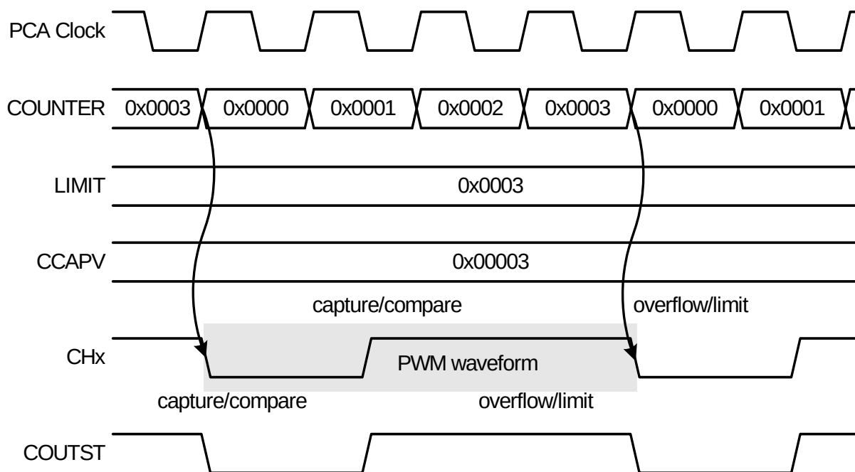
Figure 22.6. Example Edge-Aligned PWM Timing Diagram
