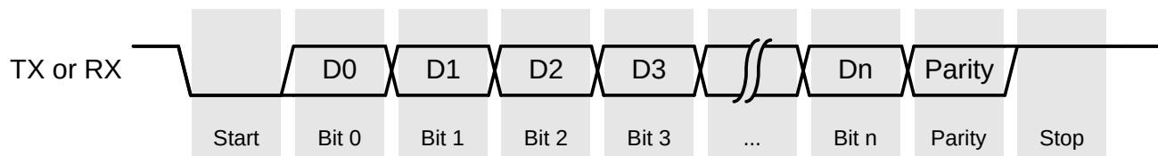
Figure 37.2. Basic Asynchronous Communication
