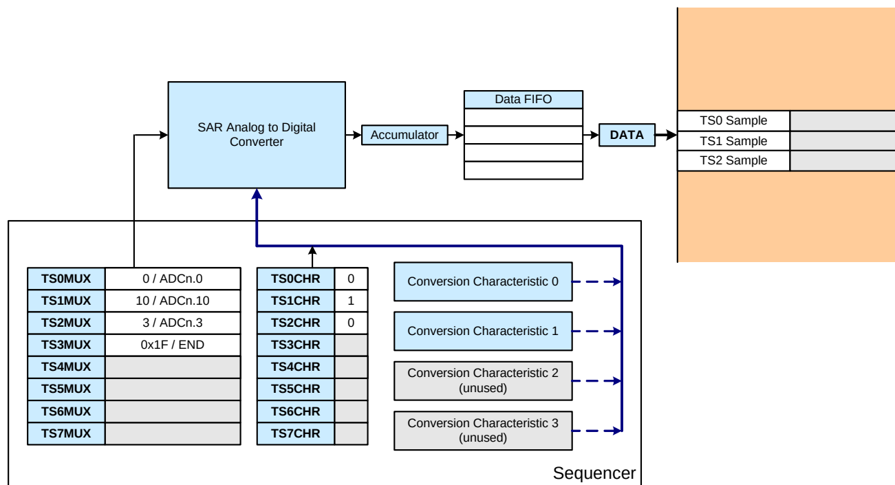
Figure 34.6. Channel Scan Setup and Timing
