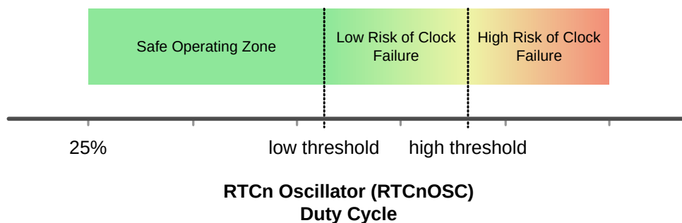
Figure 33.4. Interpreting Oscillation Robustness (Duty Cycle) Test Results
