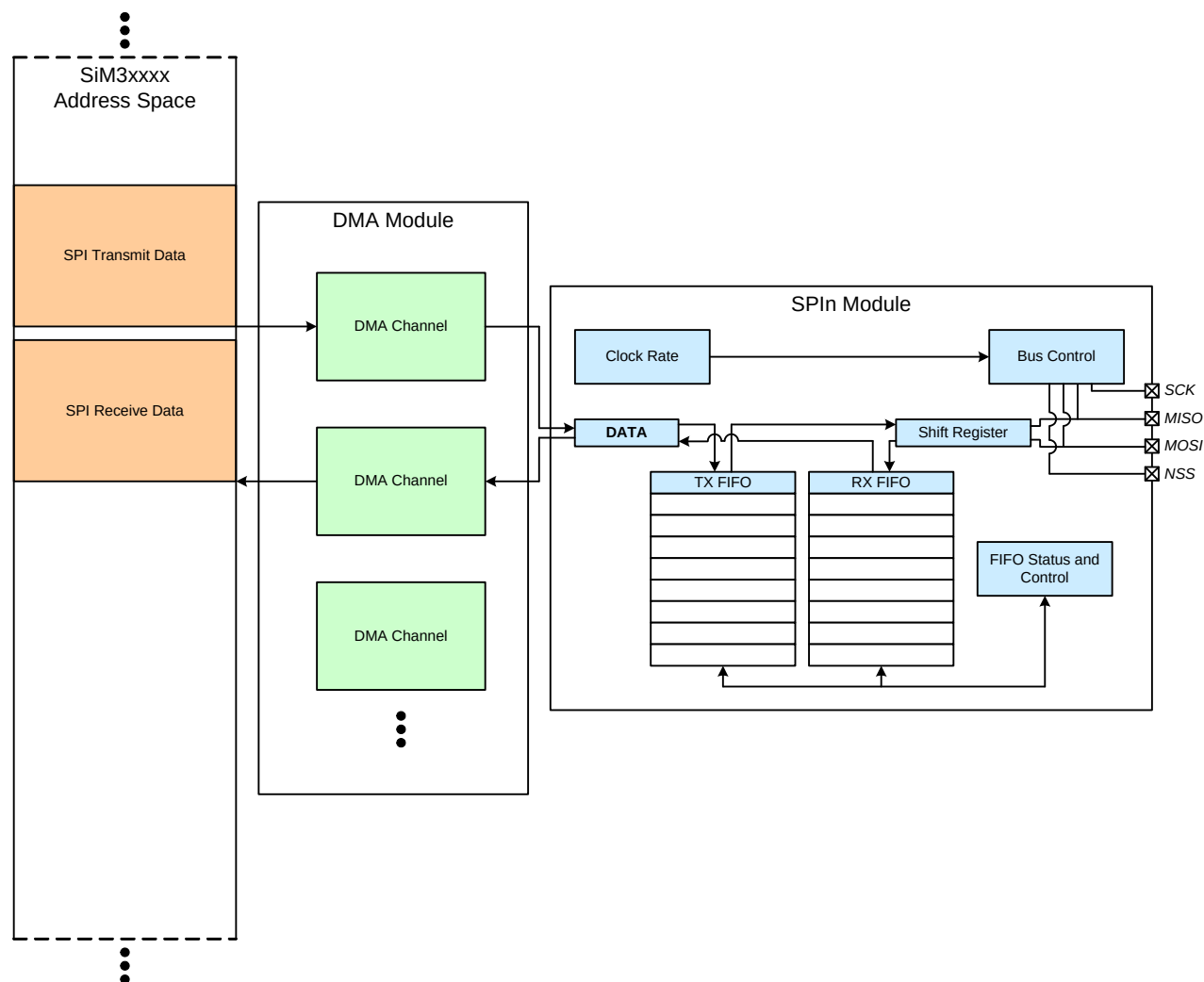
Figure 35.14. SPI DMA Configuration
