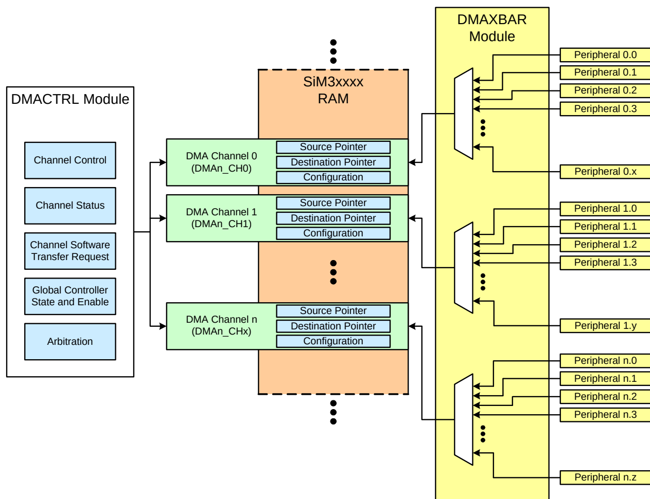
Figure 17.1. DMACTRL and DMACH Block Diagram
