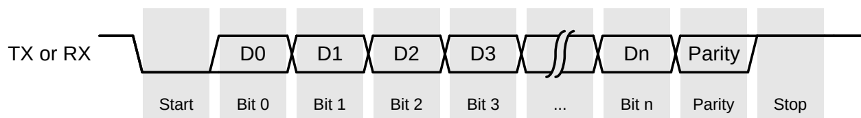
Figure 38.2. Basic Asynchronous UART Communication
