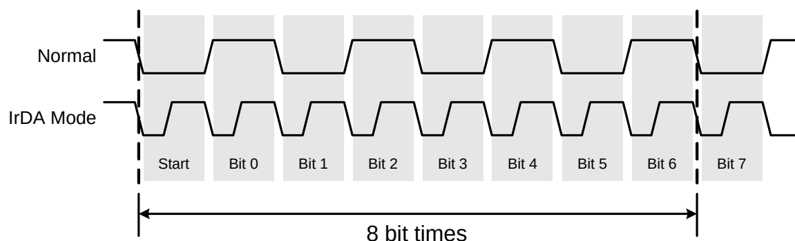
Figure 38.3. Receiver Auto-Baud Detection Input Timing
