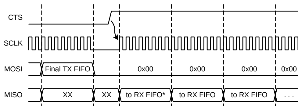
Figure 35.12. CTS Pin Polling
