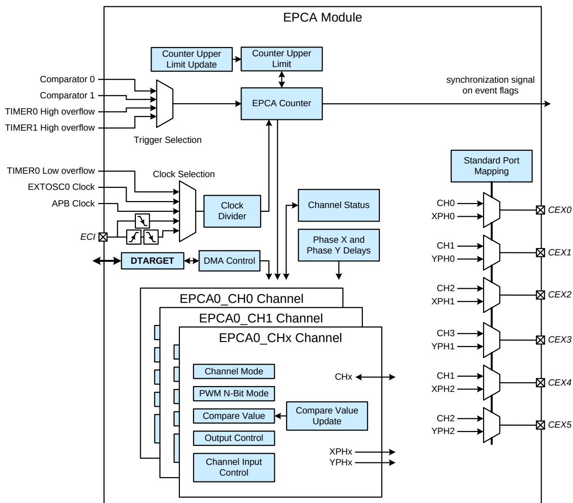
Figure 22.1. EPCA Block Diagram
