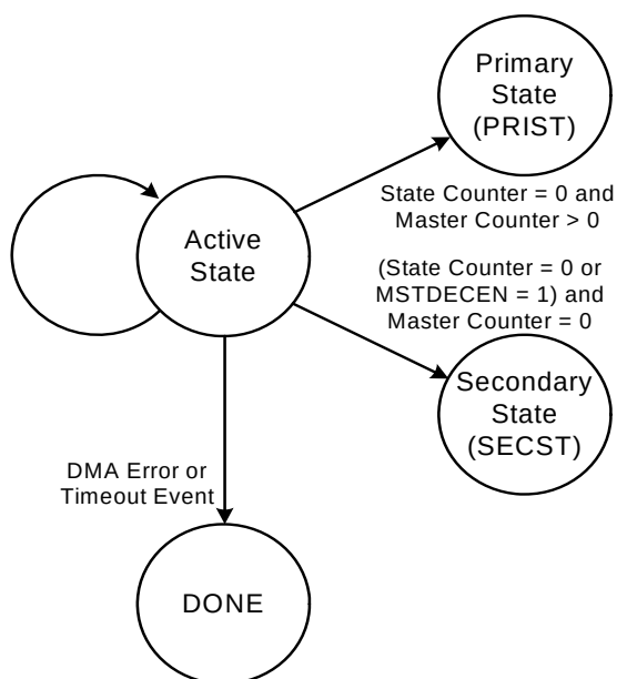
Figure 19.2. State Transition Diagram
