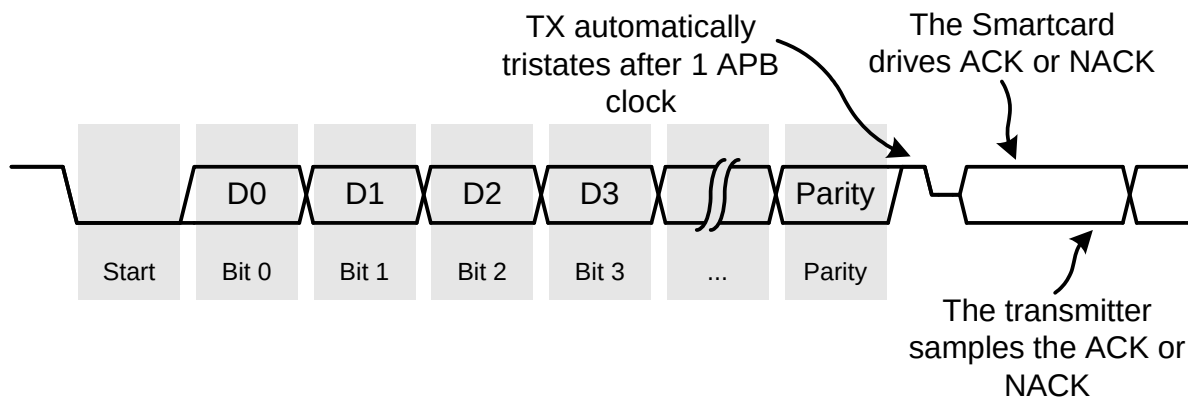
Figure 37.7. Smartcard Transmit Signalling
