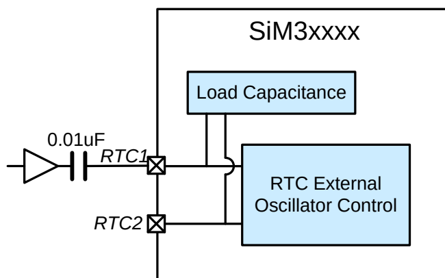
Figure 33.3. External CMOS Clock Mode Hardware Configuration
