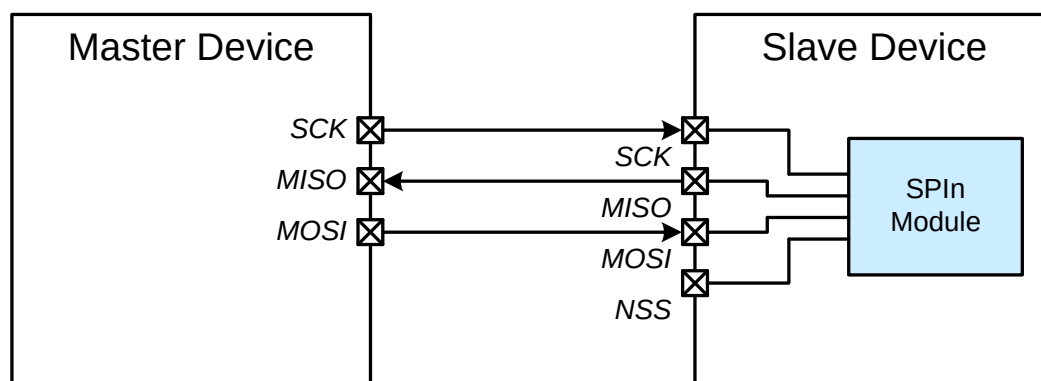
Figure 35.9. 3-Wire Single Slave Mode Connection Diagram
