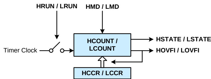
Figure 36.7. Auto-Reload Mode Block Diagram
