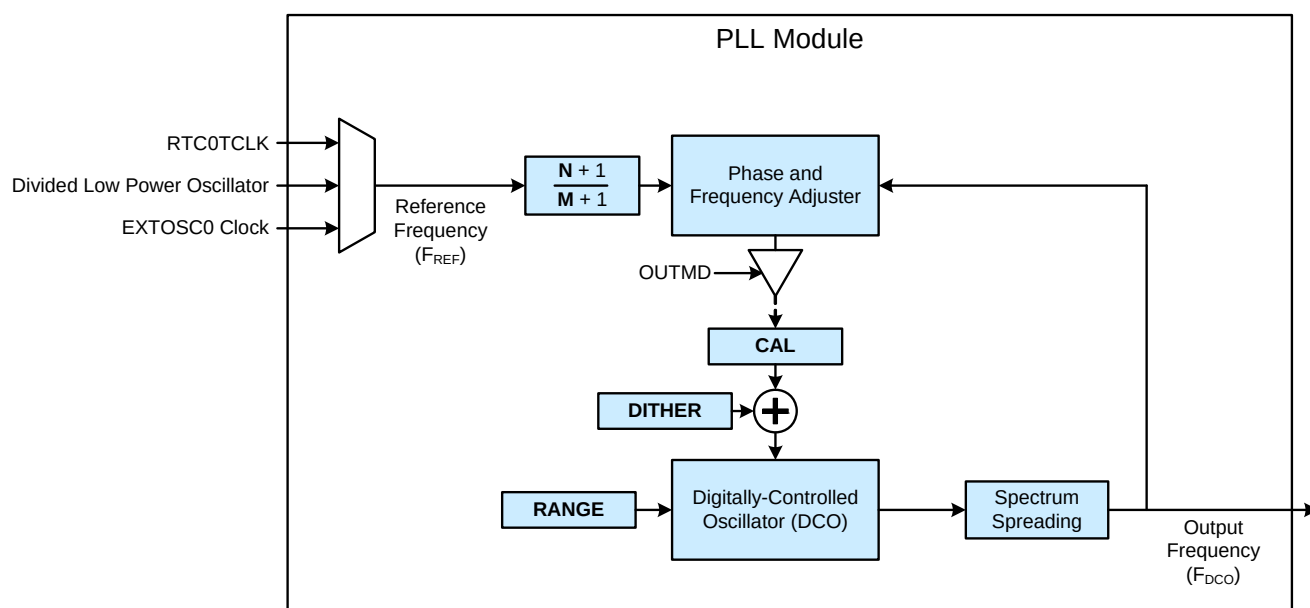
Figure 31.1. PLL Block Diagram
