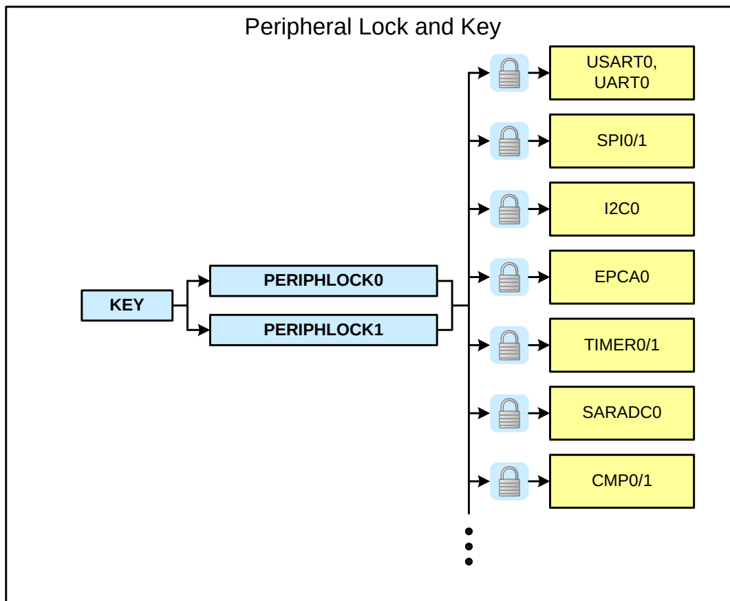
Figure 28.1. Security Block Diagram
