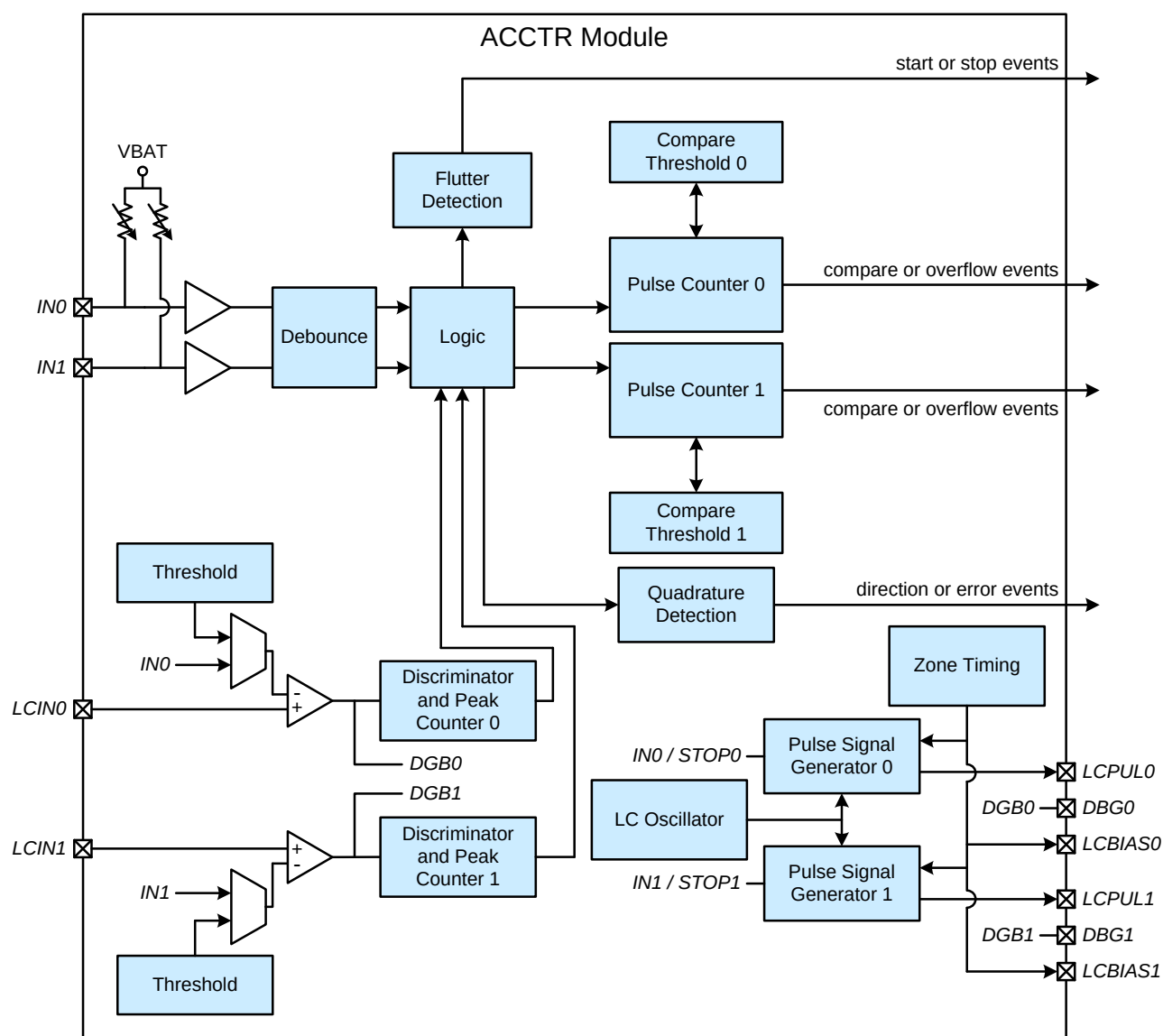
Figure 14.1. ACCTR Block Diagram
