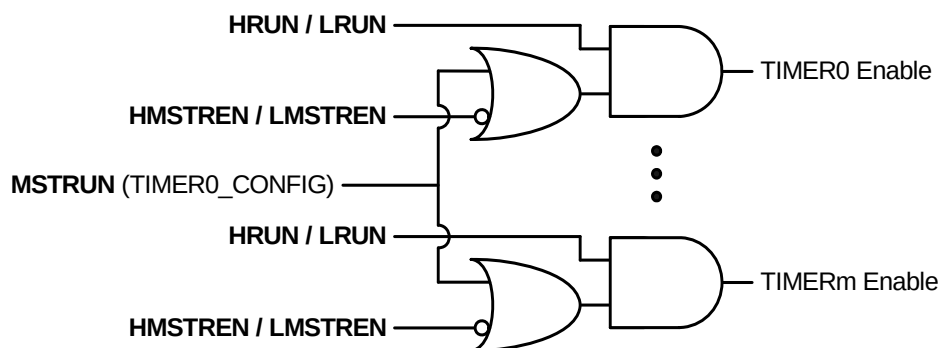
Figure 36.5. Timer Synchronization Block Diagram
