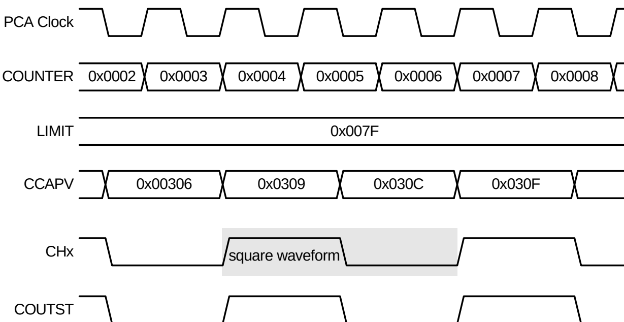
Figure 22.10. Example High-Frequency Square Wave Mode Timing Diagram
