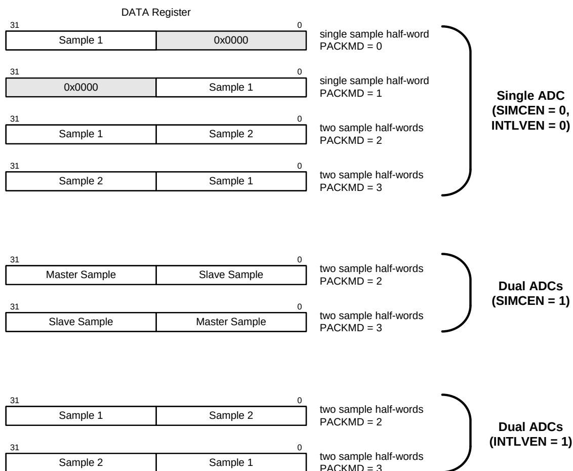
Figure 34.9. ADC Output Data Packing Options
