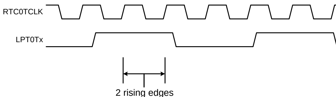
Figure 30.2. External Input Clock Synchronization Timing
