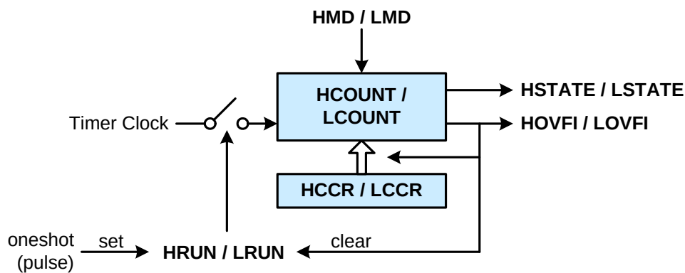
Figure 36.17. One Shot Mode Block Diagram
