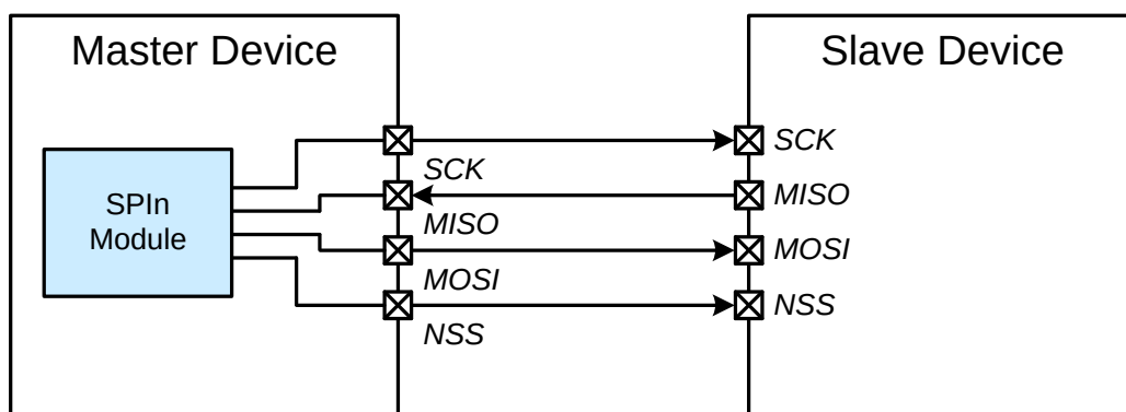
Figure 35.6. 4-Wire Single Master Mode Connection Diagram
