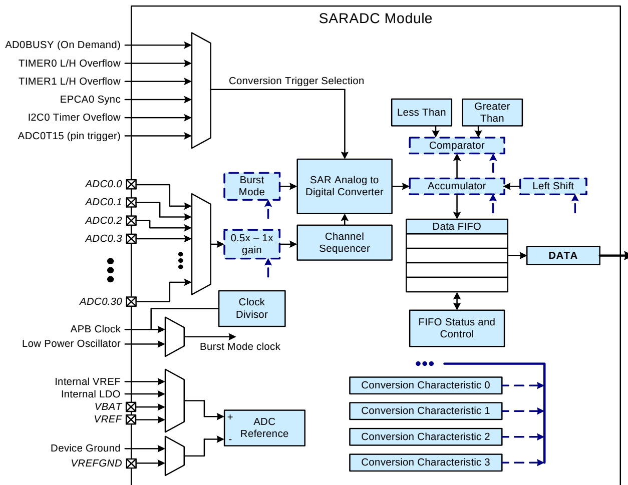
Figure 34.1. SARADC Block Diagram
