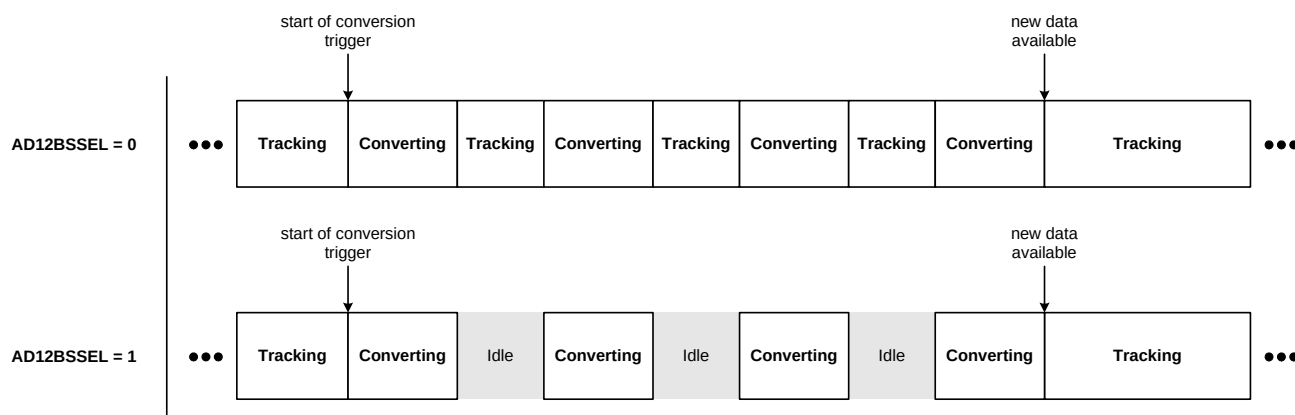
Figure 34.4. 12-Bit Sampling Options
