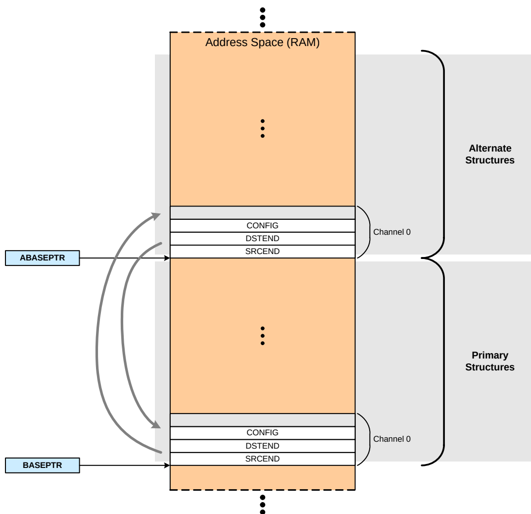
Figure 17.5. Ping-Pong Transfer Memory Configuration
