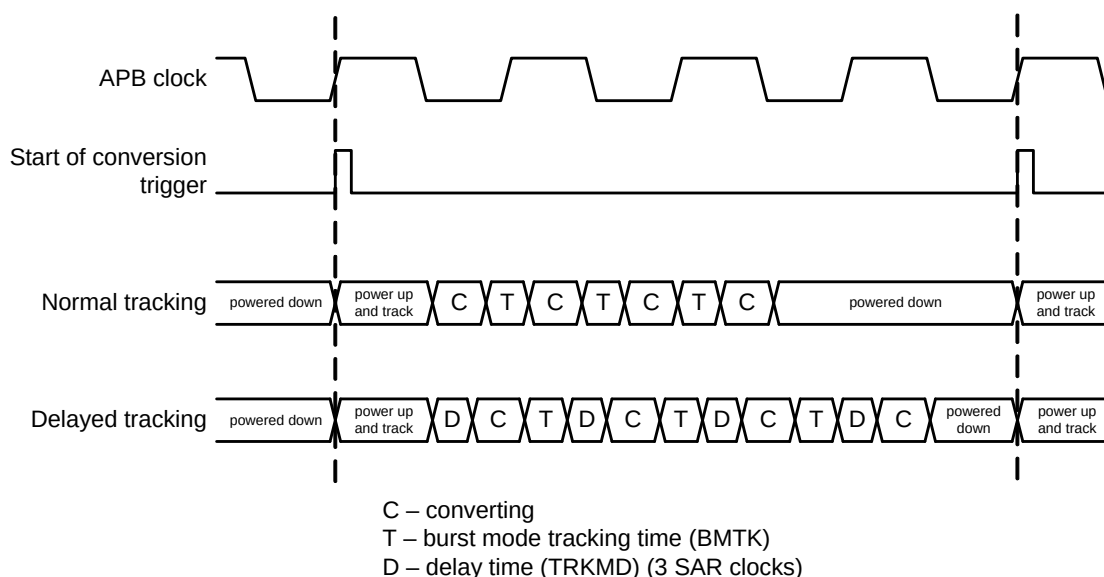
Figure 34.5. Burst Mode Tracking and Conversion Timing (Four Samples)
