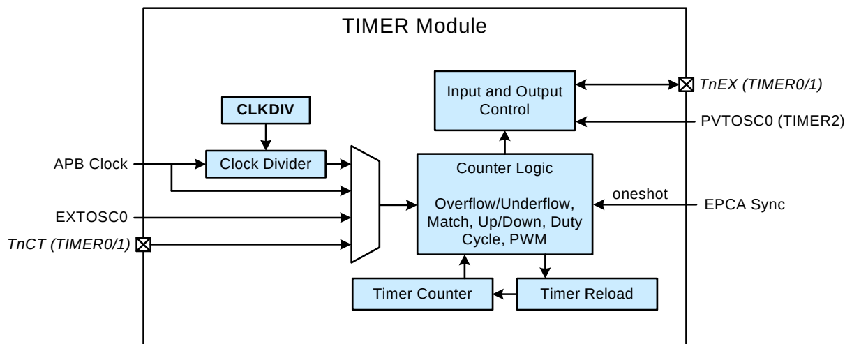
Figure 36.1. Timer Block Diagram
