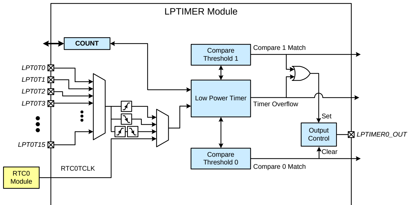
Figure 30.1. Low Power Timer Block Diagram
