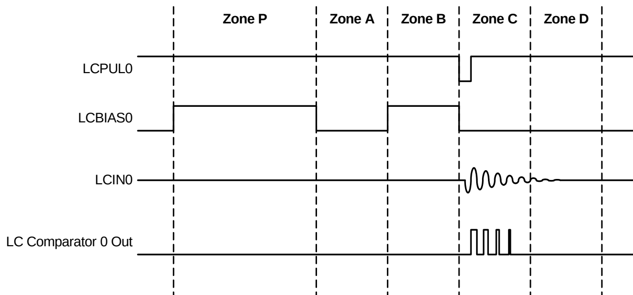
Figure 14.5. LC Resonant Timing
