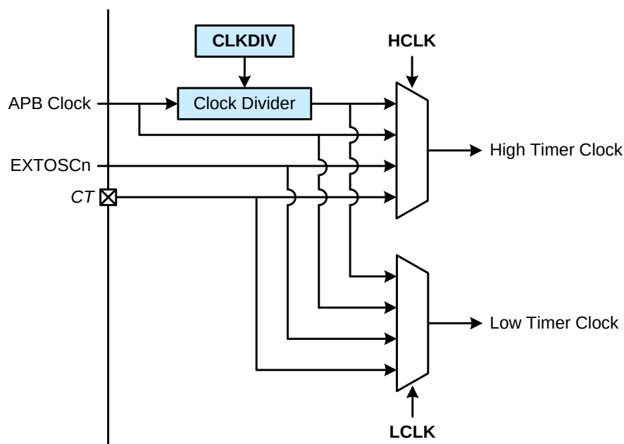
Figure 36.3. Clock Source Selection (SPLITEN = 1)
