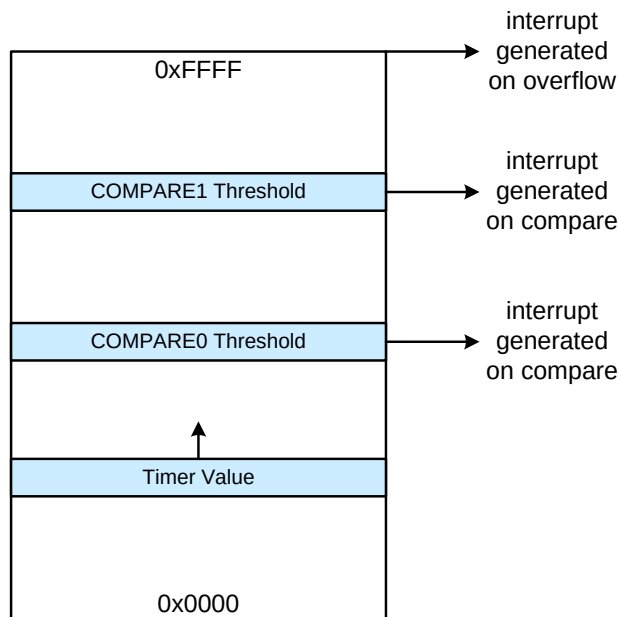
Figure 30.3. Low Power Timer Operation
