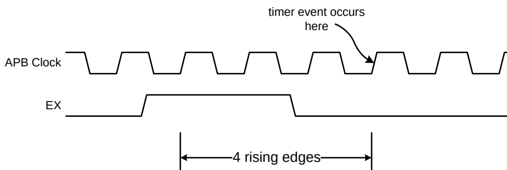
Figure 36.6. EX Signal Synchronization Timing
