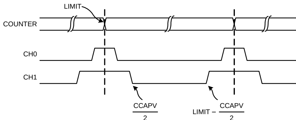
Figure 22.7. Multiple Center-Aligned PWM Channels
