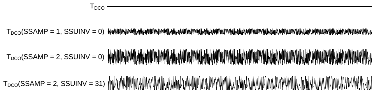
Figure 31.7. Spectrum Spreading Example
