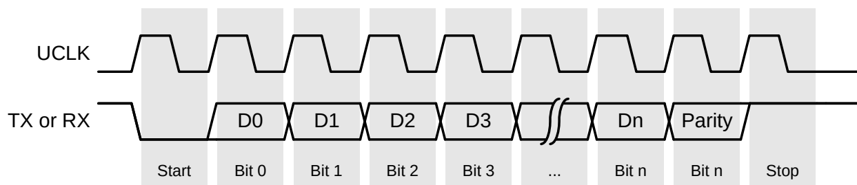
Figure 37.4. Synchronous Communication
