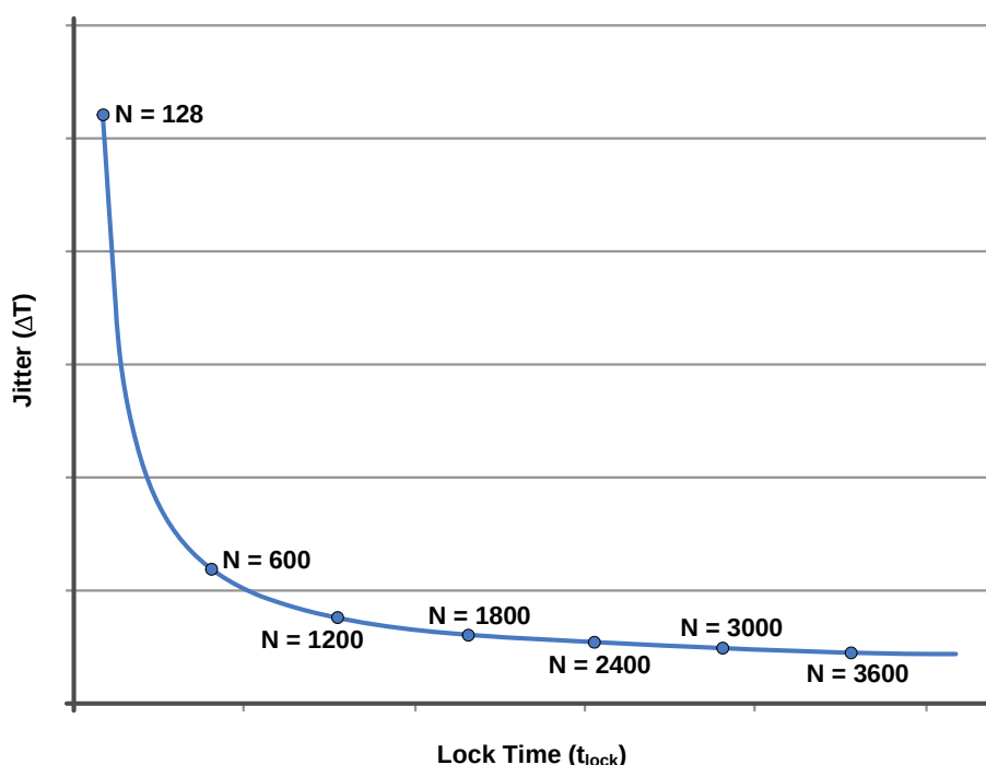
Figure 31.5. Jitter vs. Lock Time for Values of N
