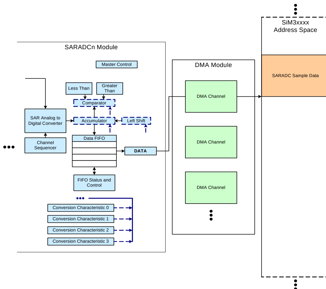
Figure 34.14. SARADC DMA Configuration
