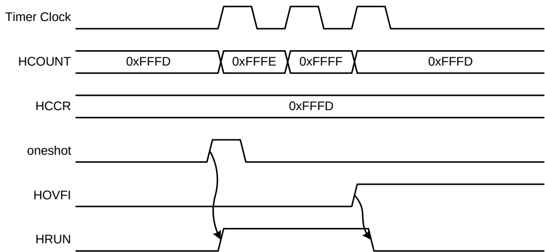
Figure 36.18. One Shot Mode Timing Diagram
