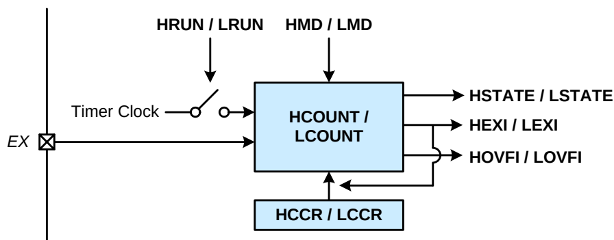
Figure 36.9. Up/Down Mode Block Diagram
