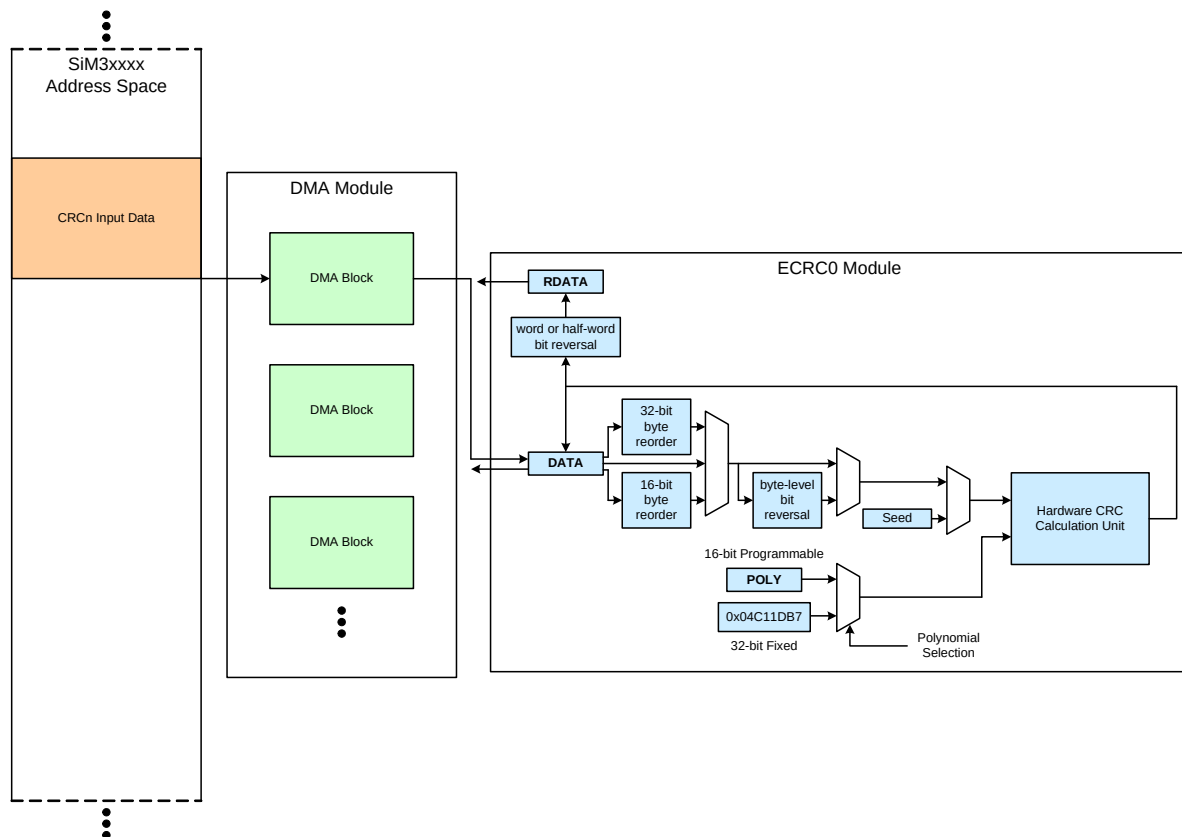
Figure 20.3. DMA Configuration
