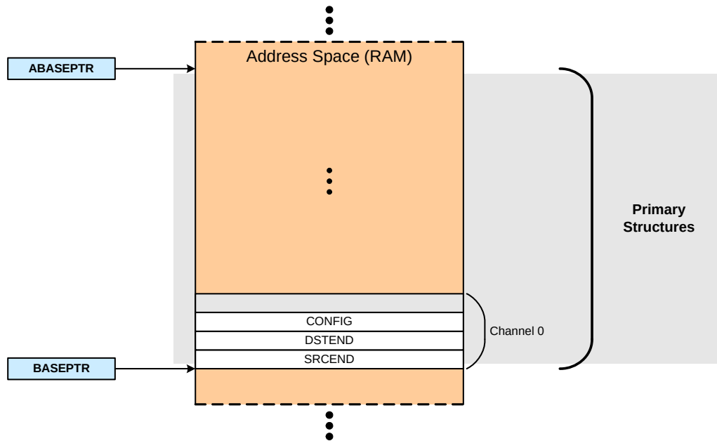
Figure 17.3. Basic and Auto-Request Transfer Memory Configuration
