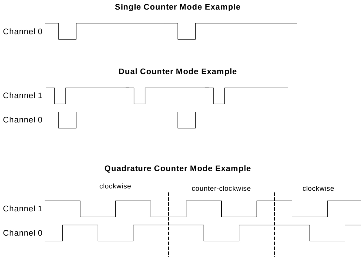
Figure 14.6. Counter Mode Examples
