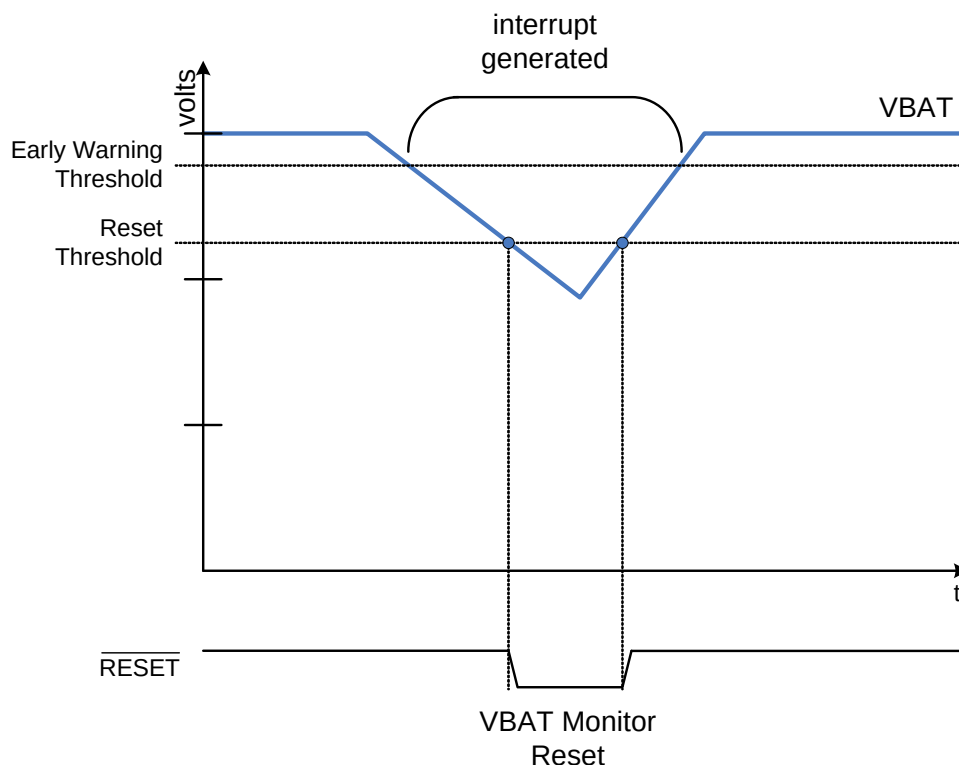
Figure 39.2. VBAT Supply Monitor Thresholds
