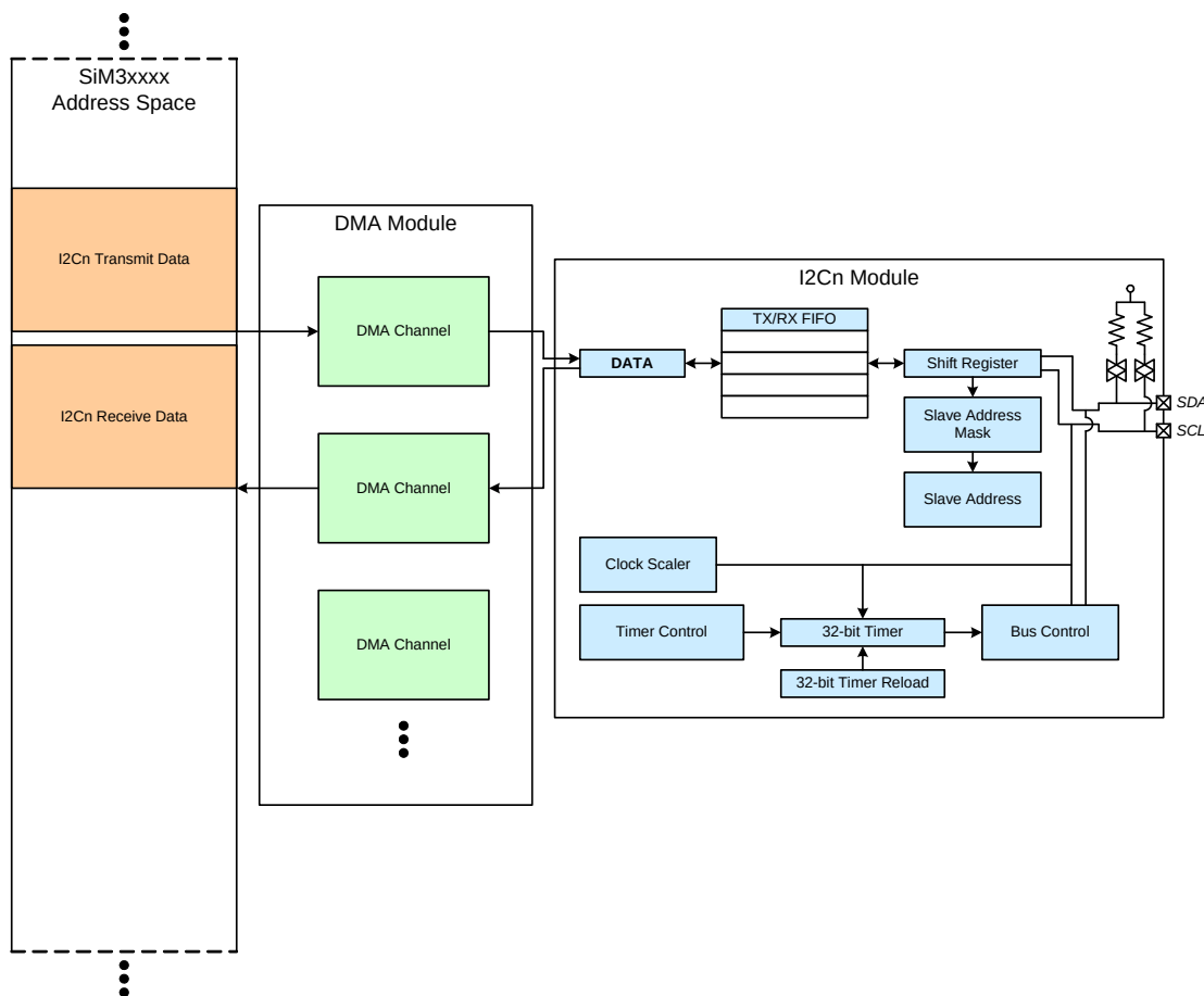
Figure 25.16. I2C Module DMA Configuration
