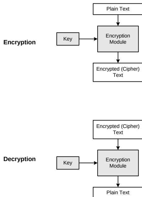
Figure 15.3. Electronic Codebook (ECB) Algorithm Diagram
