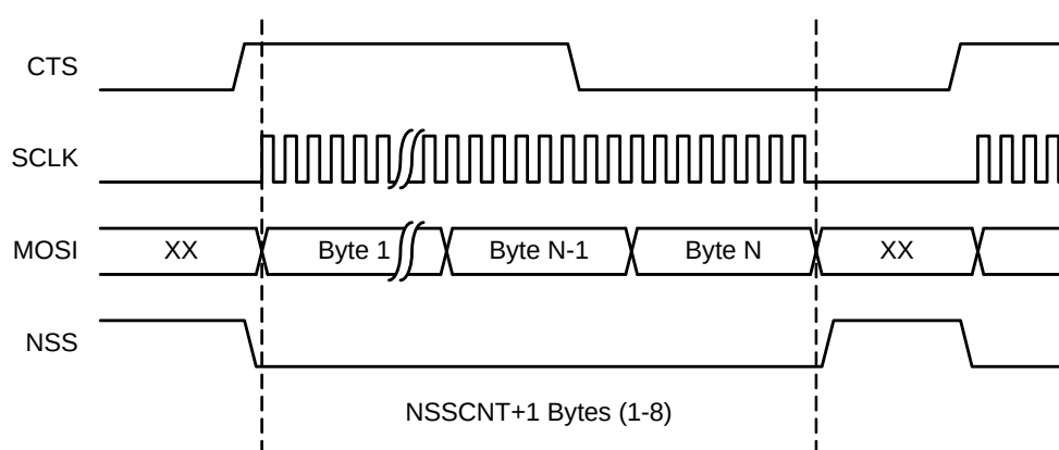
Figure 35.13. Transmit On Request Mode Timing
