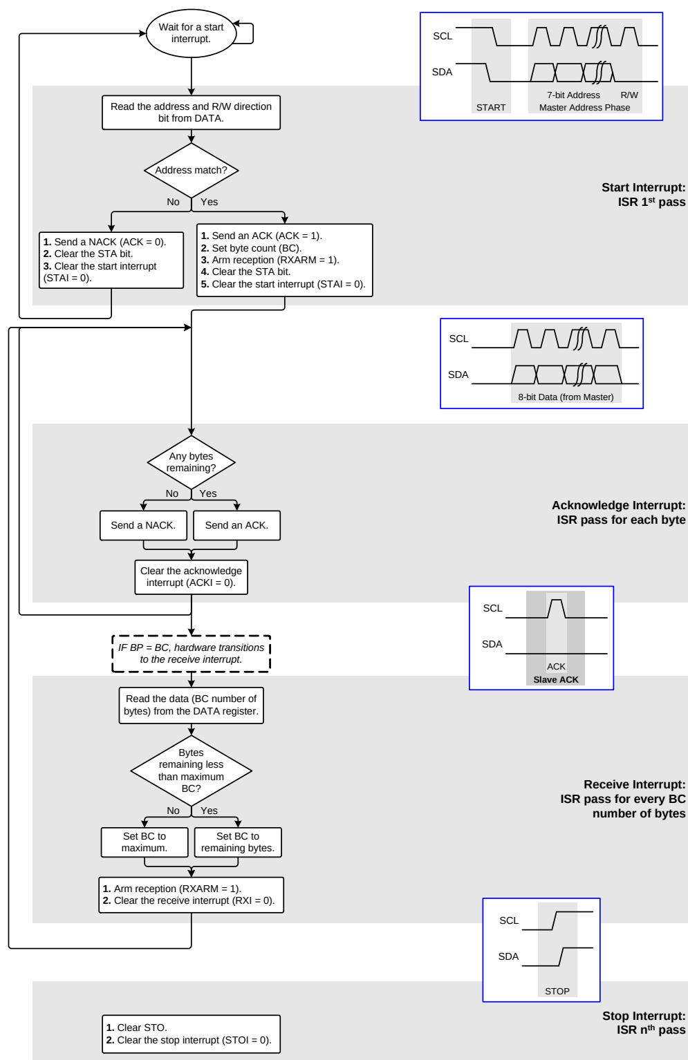
Figure 25.14. Slave Write Flow Diagram (7-bit Address)
