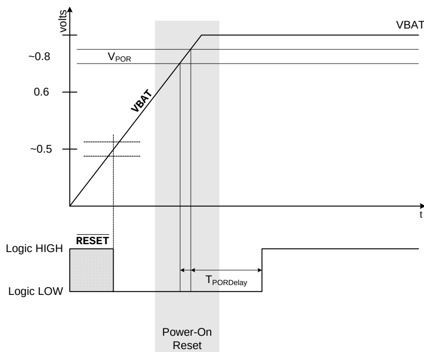
Figure 7.2. Power-On Reset Timing Diagram
