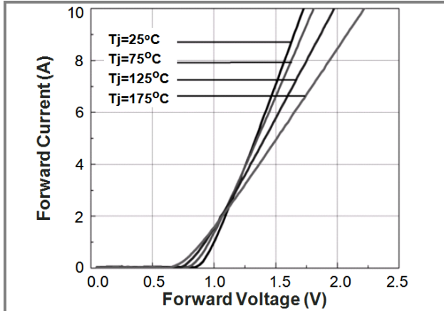
Fig.1 Forward Characteristics
