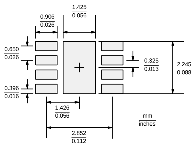
Figure 7. MLP33 PowerPAK Pad Pattern
