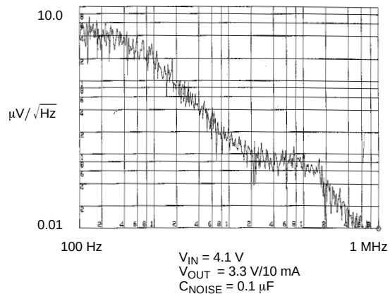
Noise Spectrum
