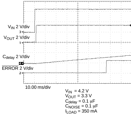
Turn-On Sequence
