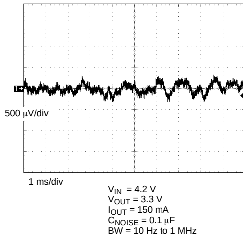
Output Noise
