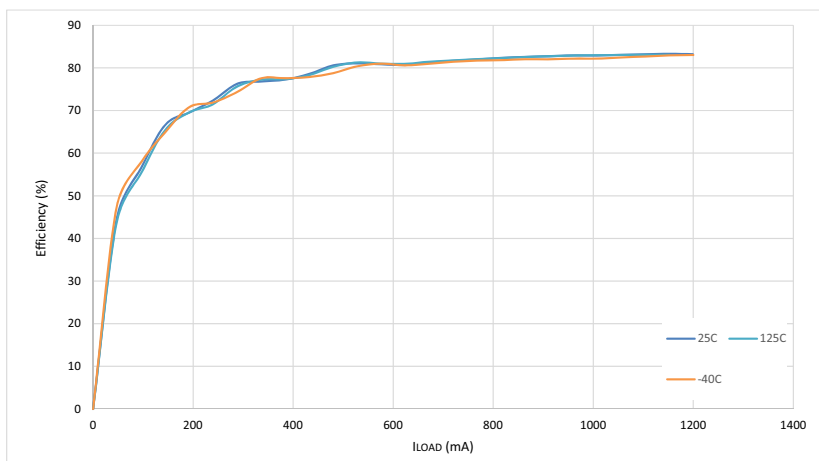
Figure 17. Efficiency vs. Load Current over Temperature (24 V to 5 V)
