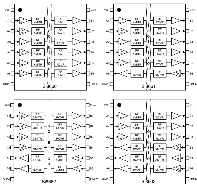
Figure 5.1. Si866x Pinout
