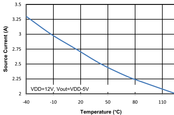
Figure 31. Output Source Current vs. Temperature
