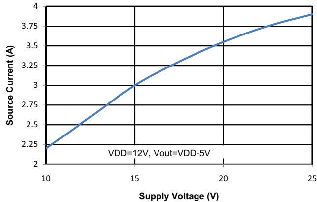
Figure 29. Output Source Current vs. Supply Voltage
