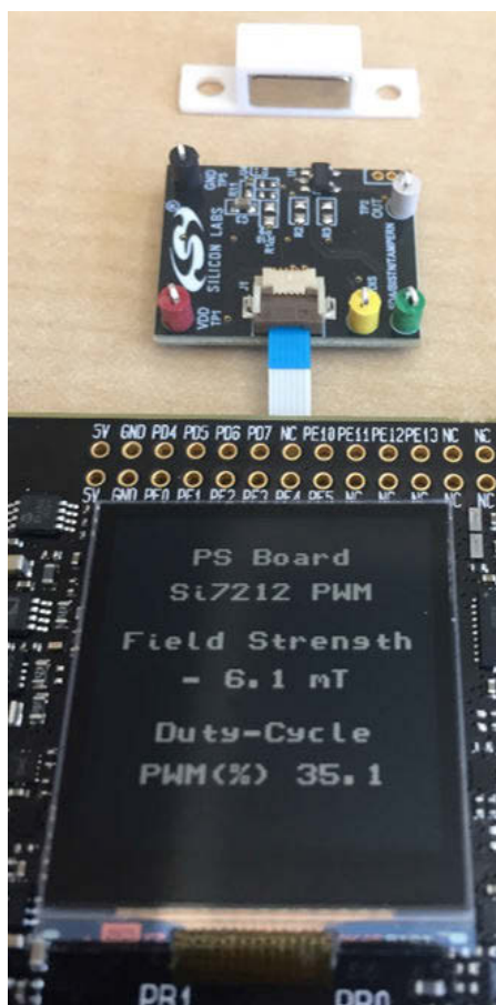
Figure 1.11. PWM Screen
