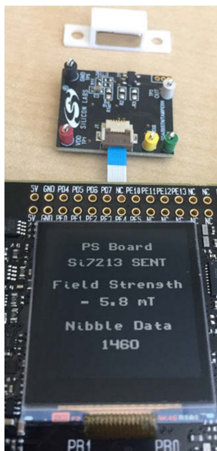
Figure 1.12. Sent Screen
