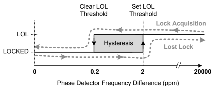
Figure 3.12. LOL Set and Clear Thresholds
