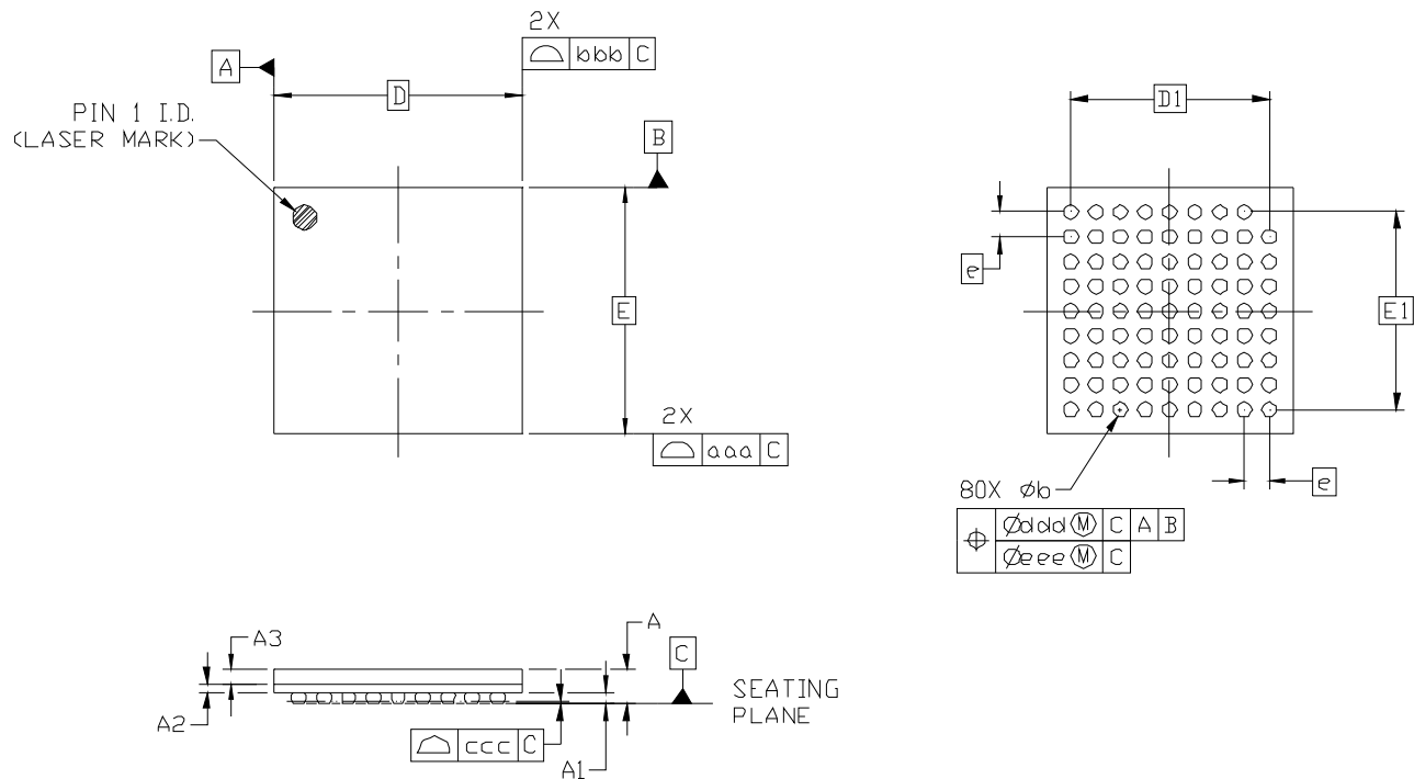
Figure 11. 80-Pin Plastic Ball Grid Array (PBGA)
