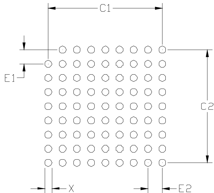
Figure 12. PBGA Card Layout
