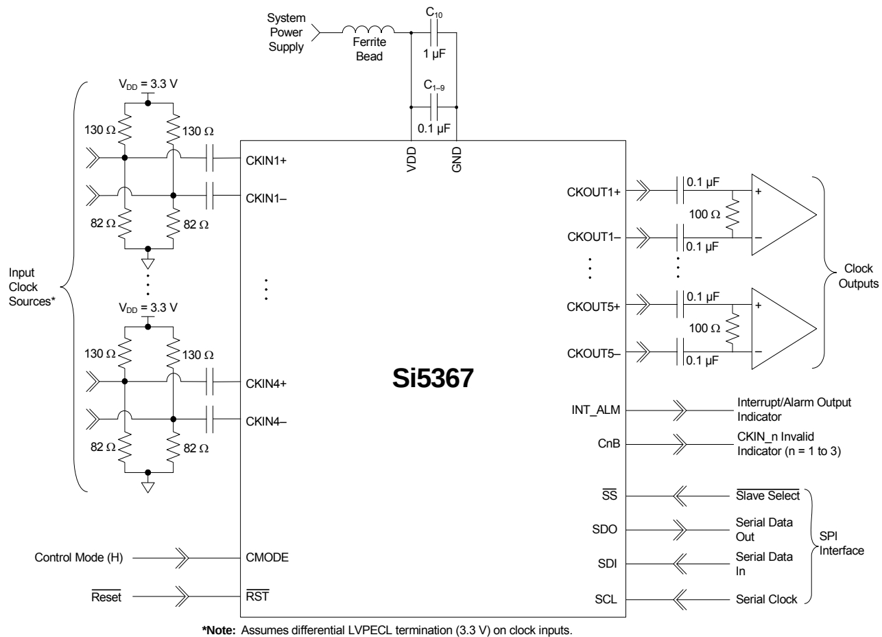
Figure 5. Si5367 Typical Application Circuit (SPI Control Mode)
