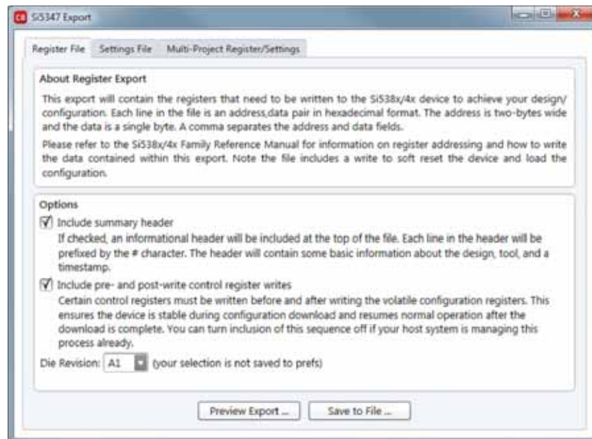
Figure 27. Export Settings
