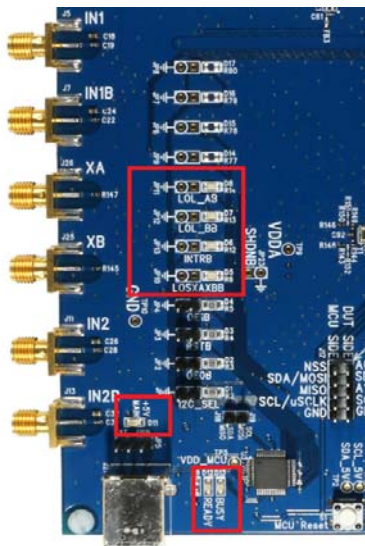
Figure 3. Status LEDs
