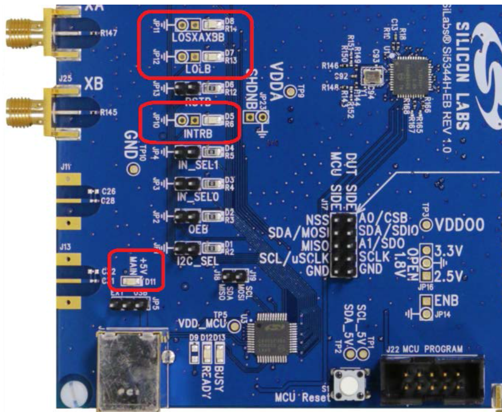
Figure 1.2. Status LEDs
