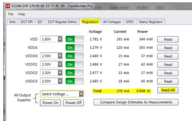
Figure 15. EVB GUI Window
