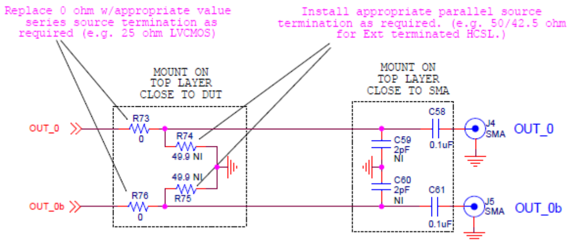
Figure 3.4. Si5332-6A-EVB Single Pair Output Clock Termination Circuit
