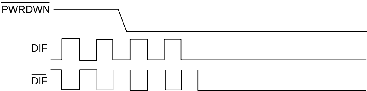
Figure 1. \overline{\text{PWRDN}} Assertion
