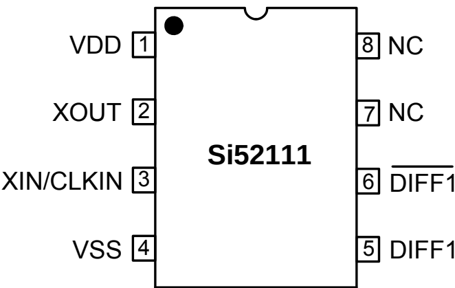
Figure 7. 8-Pin TSSOP
