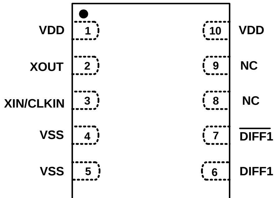
Figure 6. 10-Pin TDFN
