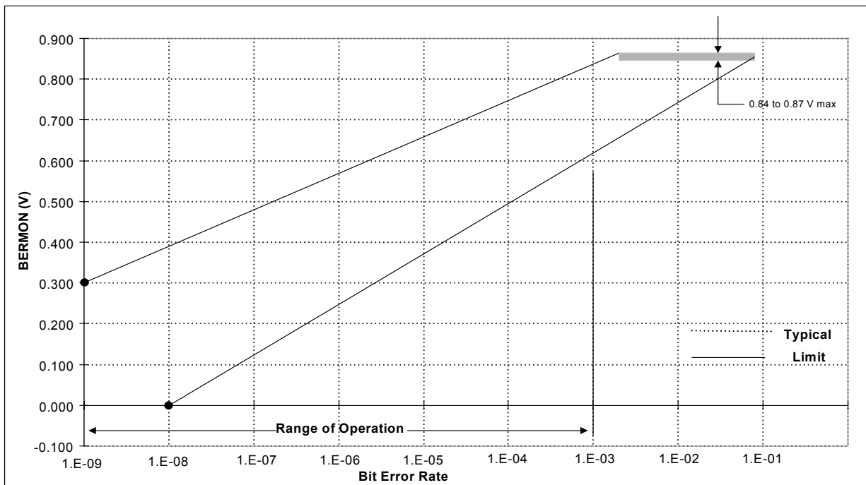
Figure 10. Si5023 OC-12/OC-3 BERMON Voltage Characteristics
