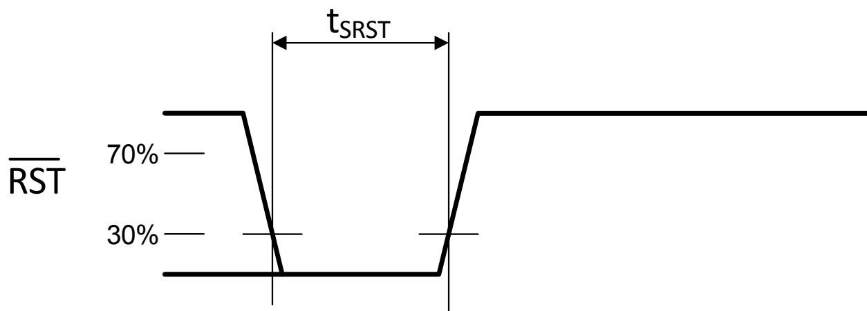
Figure 1. Reset Timing
