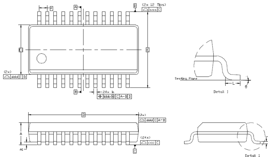
Figure 5. 24-Pin SSOP
