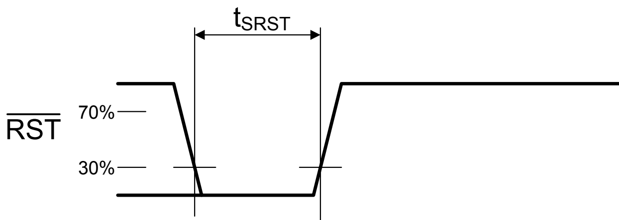
Figure 1. Reset Timing
