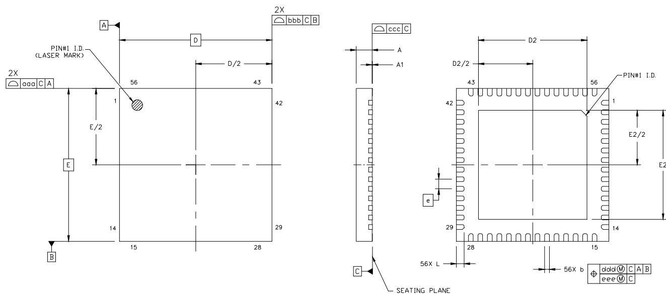
Figure 13. Package Drawing
