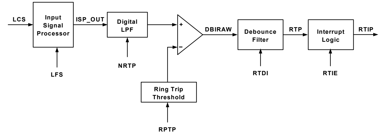
Figure 14. Ring Trip Detector
