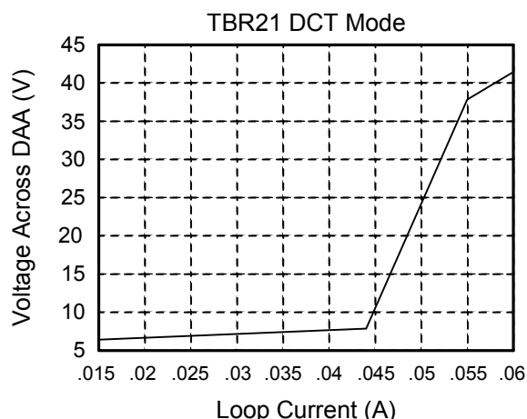
Figure 22. TBR21 Mode I/V Characteristics, DCV[1:0] = 11, MINI[1:0] = 00, ILIM = 1
