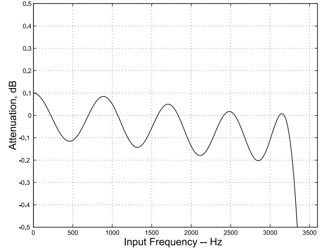
Figure 10. FIR Transmit Filter Passband Ripple
