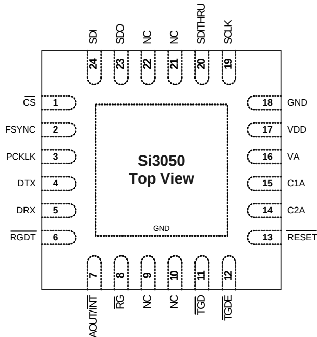
Figure 50. Si3050 QFN
