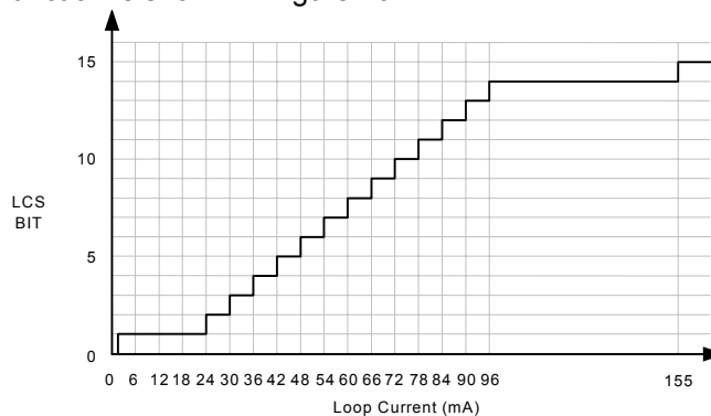
Figure 26. Typical LCS Transfer Function
