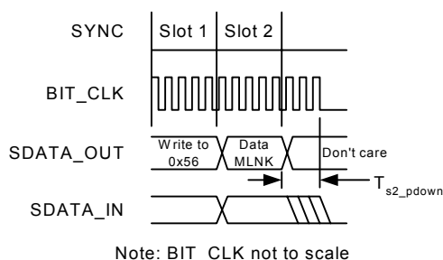
Figure 7. AC-Link Low Power Mode Timing Diagram
