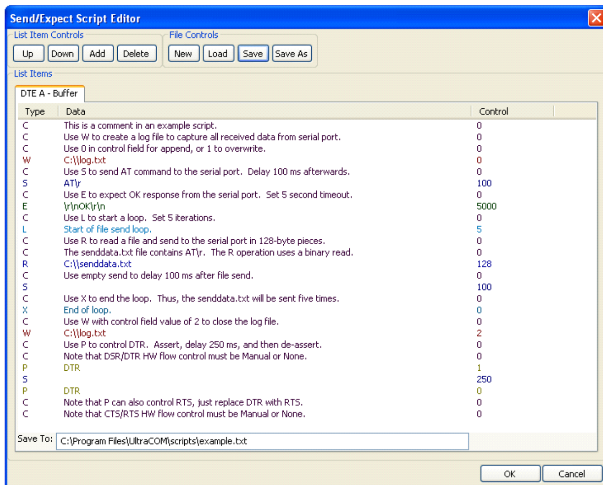
Figure 72. UltraCOM Script Editor
