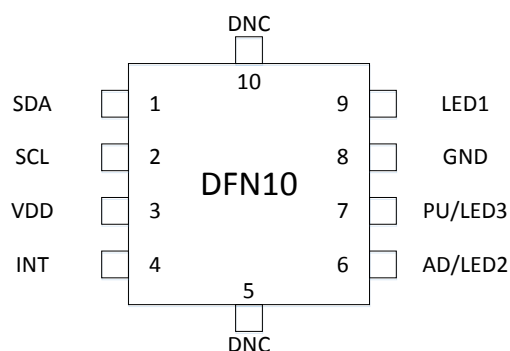
Figure 9.1. 10-Pin DFN
