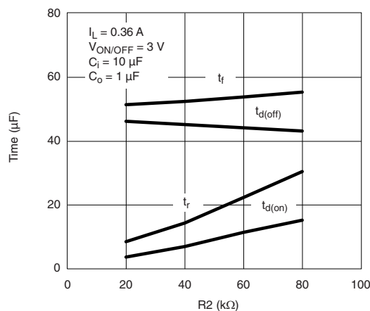
Switching Variation R2 at V_{IN} = 2.5 V , R1 = 300 k\Omega
