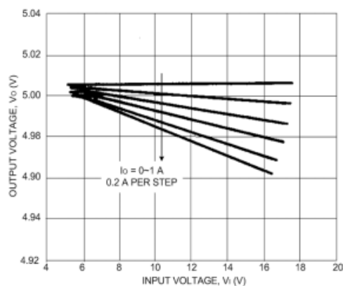
■ Line Regulation
