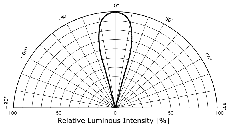
Fig. 5 Radiation Diagram
