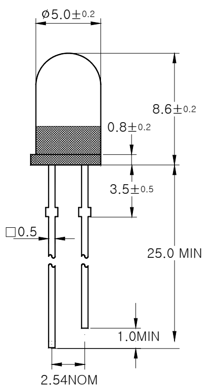
STOPPER TYPE
