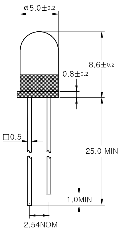
STRAIGHT TYPE
