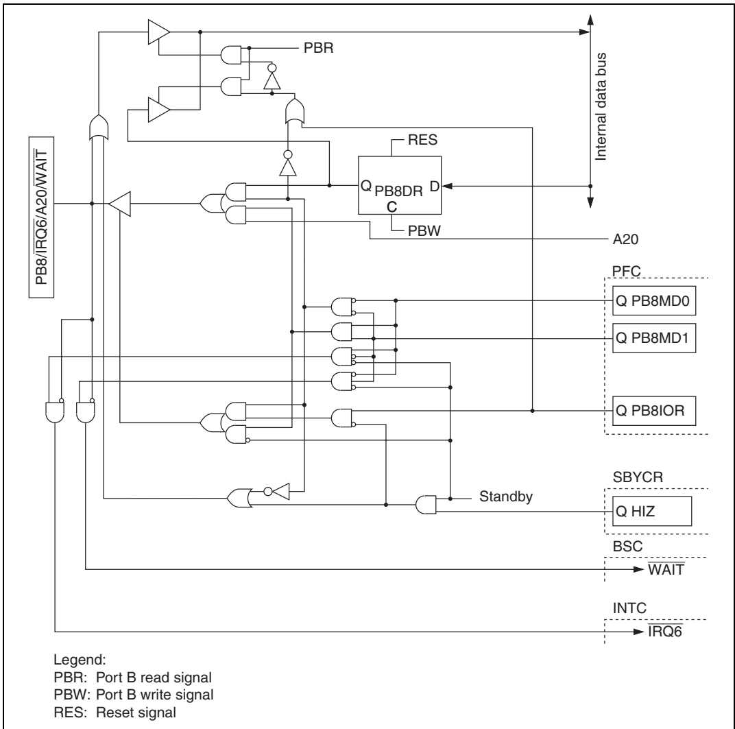
Figure B.14 PB8/ \overline{\text{IRQ6}} /A20/ \overline{\text{WAIT}} Block Diagram
