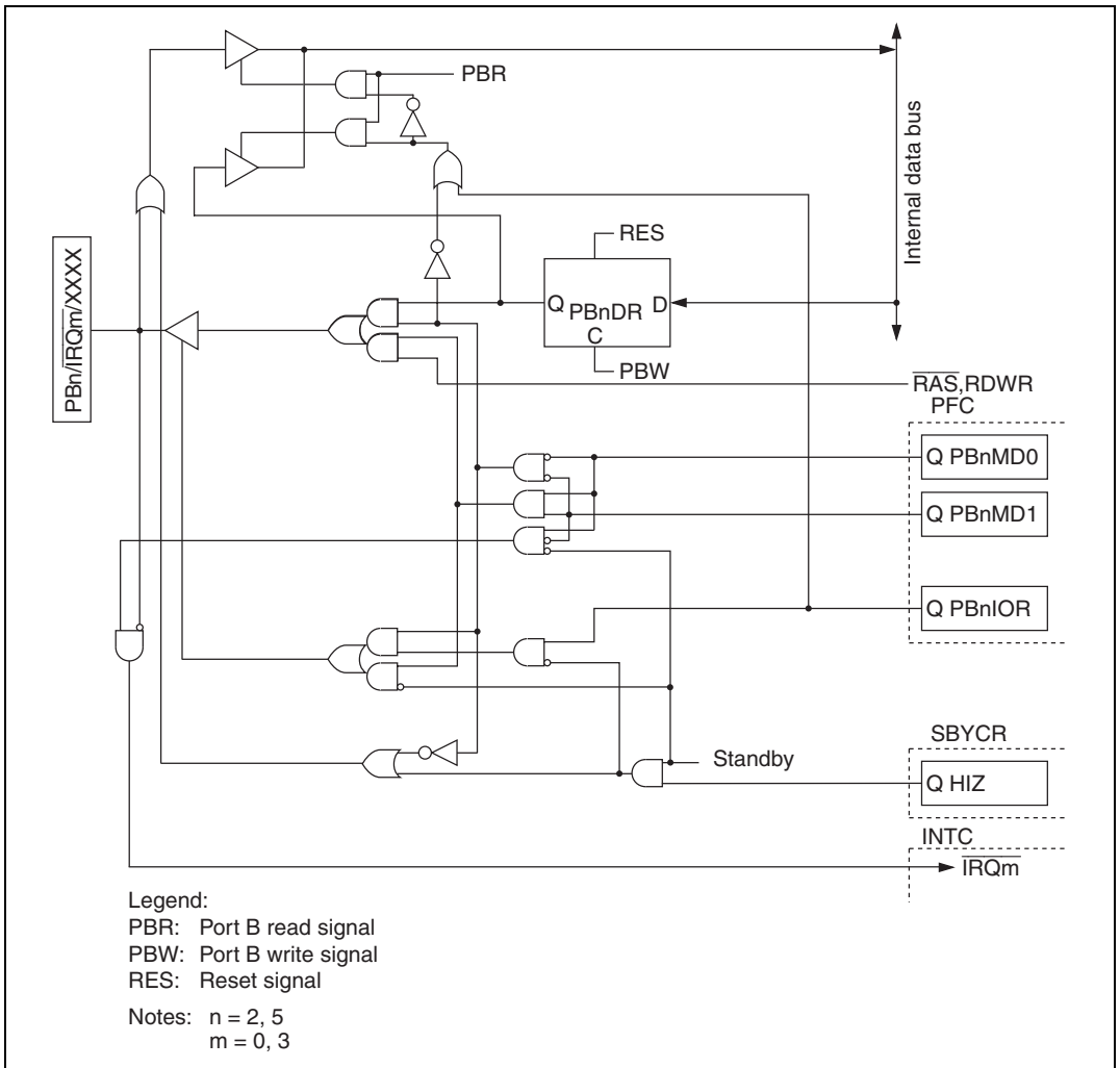
Figure B.16 \overline{\text{PBn/IRQm/XXXX}} Block Diagram
