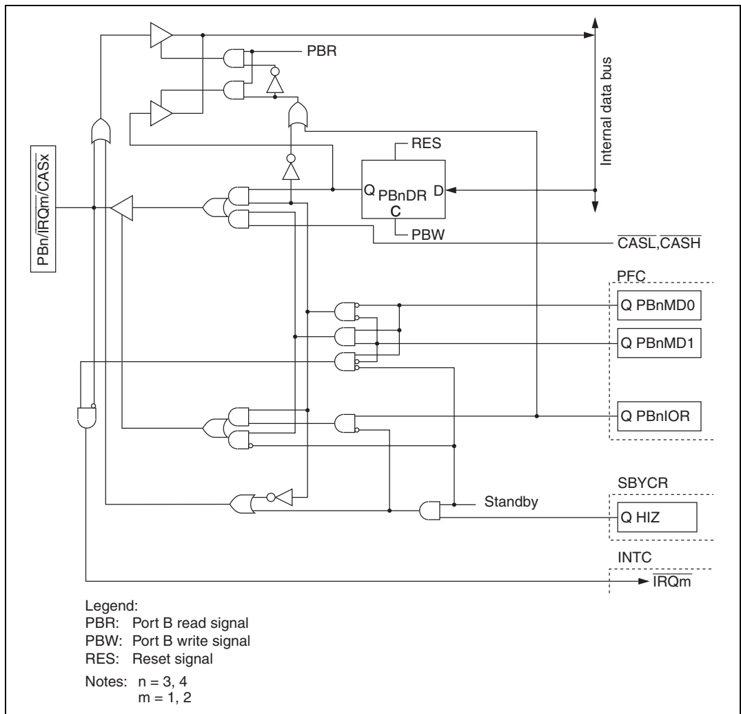
Figure B.13 PBN/ \overline{\text{IRQm}}/\overline{\text{CASx}} Block Diagram
