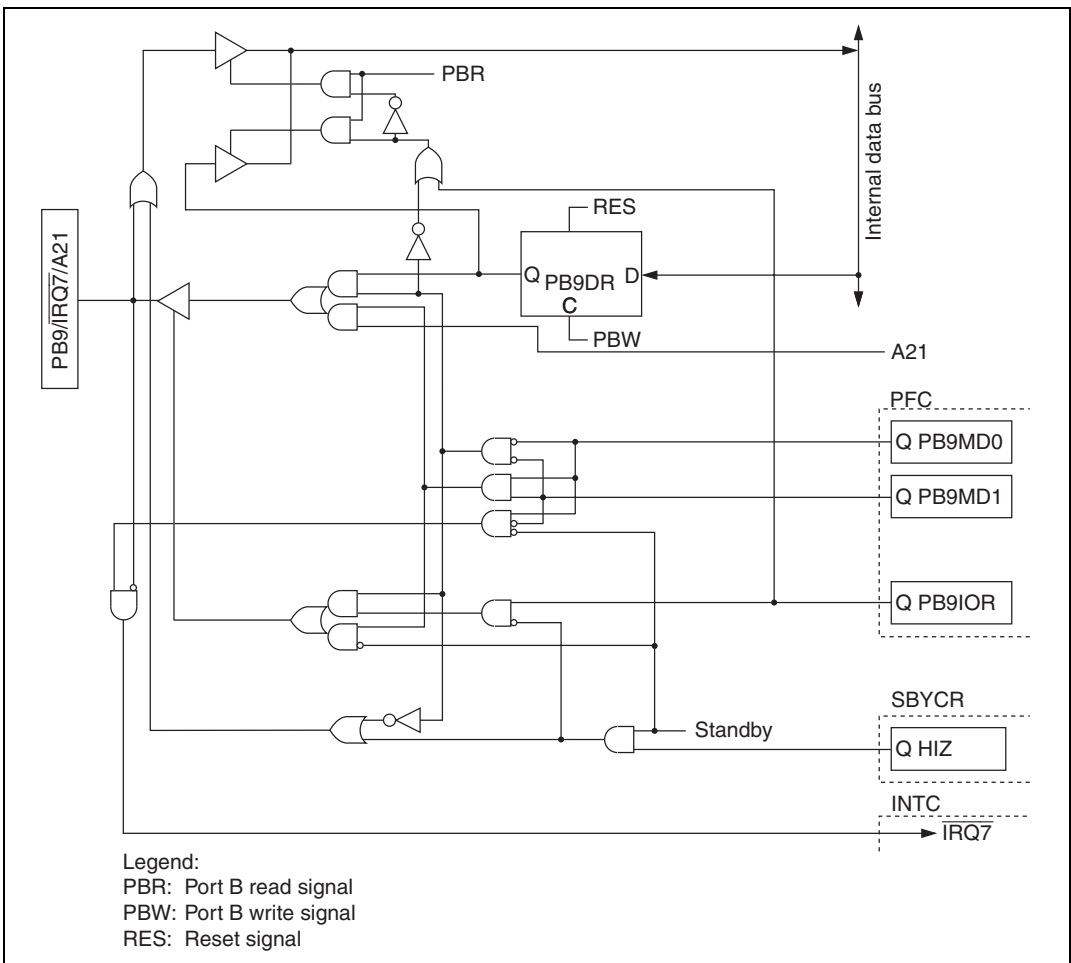
Figure B.15 PB9/TRQ7/A21 Block Diagram
