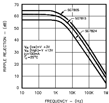
FIGURE 3. RIPPLE REJECTION VS. FREQUENCY
