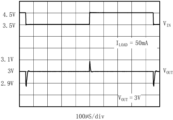
Line-Transient Response
