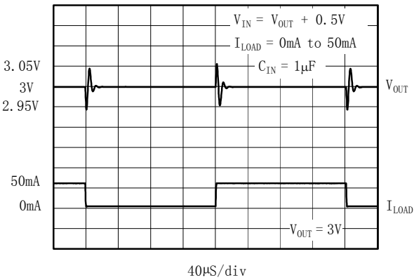
Load-Transient Response
