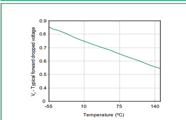
Figure 6 - Forward Voltage
