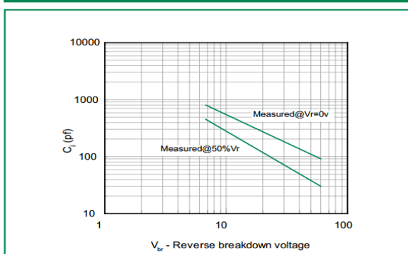
Figure 7 - C j vs. Working Peak Reverse Voltage
