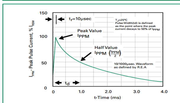
Figure 4 - Pulse Waveform - 10x1000μS
