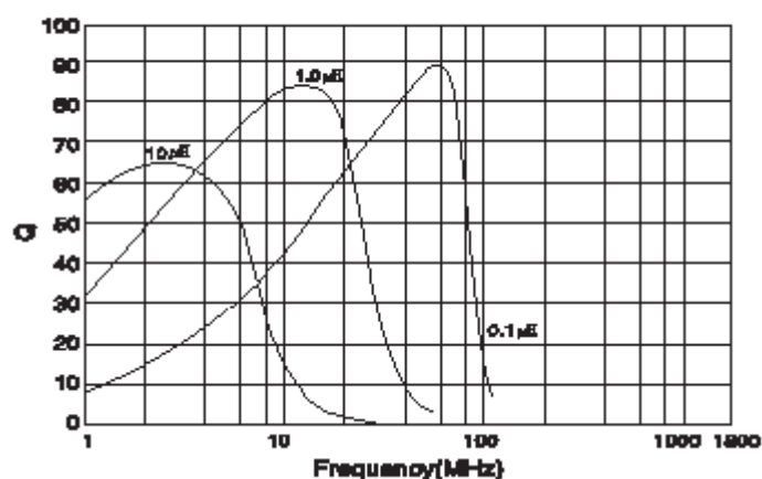
Q characteristics
