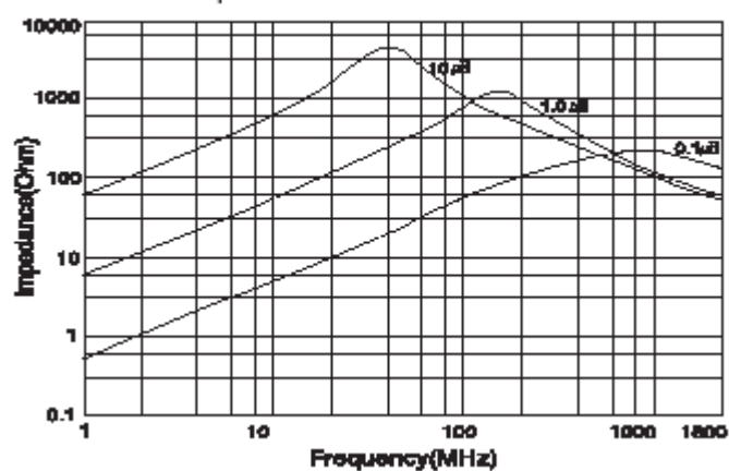
Impedance characteristics
