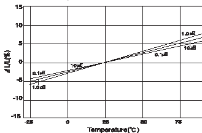
Temperature characteristics
