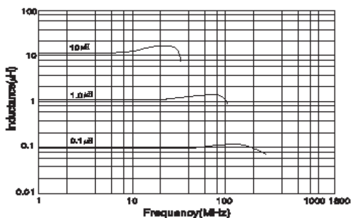
Inductance characteristics
