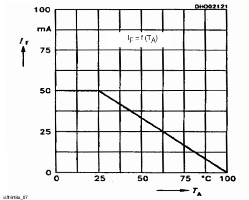
Fig. 9 Permissible Forward Current Diode
