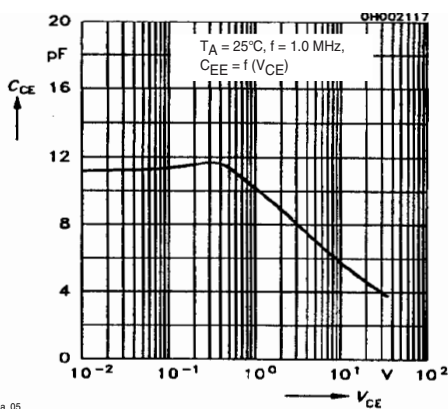
Fig. 7 Transistor Capacitance
