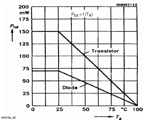
Fig. 10 Permissible Power Dissipation
