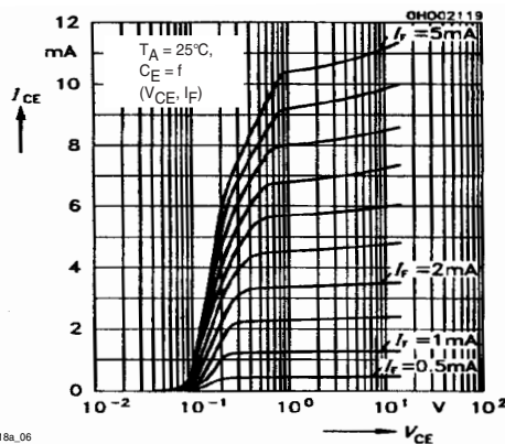
Fig. 8 Output Characteristics
